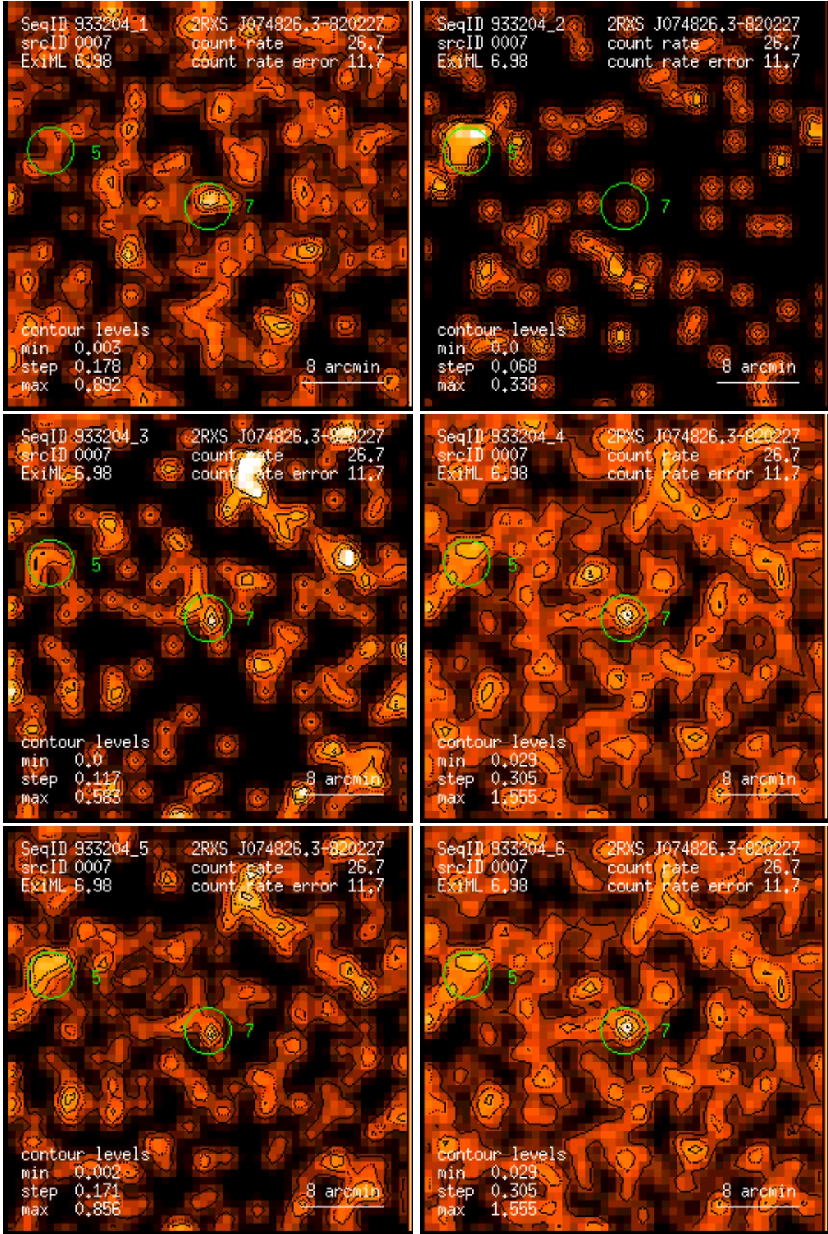
Figure 7: RASS 933204: detection 0007: band rate images, Gaussian filter: (1) PSPC channels 11 – 41, (2) 52 – 90, (3) 91 – 201, (4) 11 – 235, (5) 52 – 201, (6) 11 – 201. Broad band rates in counts/ks. Band rate contour levels in counts/ks/arcmin 2 .
