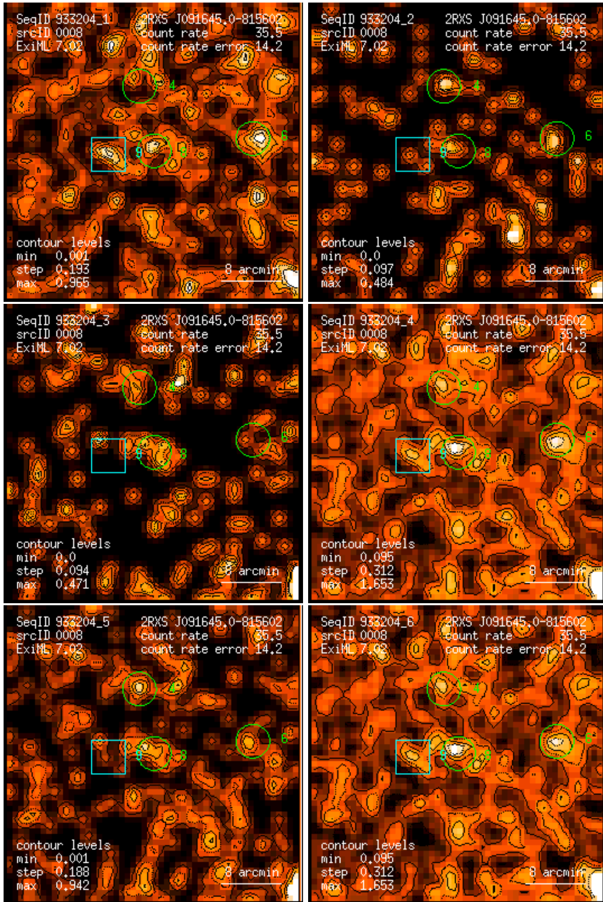
Figure 8: RASS 933204: detection 0008: band rate images, Gaussian filter: (1) PSPC channels 11 – 41, (2) 52 – 90, (3) 91 – 201, (4) 11 – 235, (5) 52 – 201, (6) 11 – 201. Broad band rates in counts/ks. Band rate contour levels in counts/ks/arcmin 2 .
