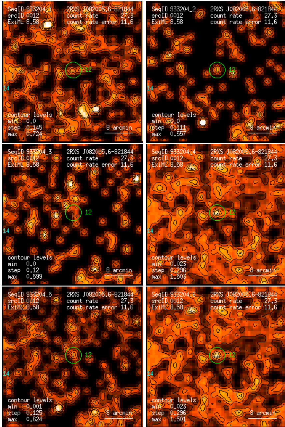
Figure 12: RASS 933204: detection 0012: band rate images, Gaussian filter: (1) PSPC channels 11 – 41, (2) 52 – 90, (3) 91 – 201, (4) 11 – 235, (5) 52 – 201, (6) 11 – 201. Broad band rates in counts/ks. Band rate contour levels in counts/ks/arcmin 2 .
