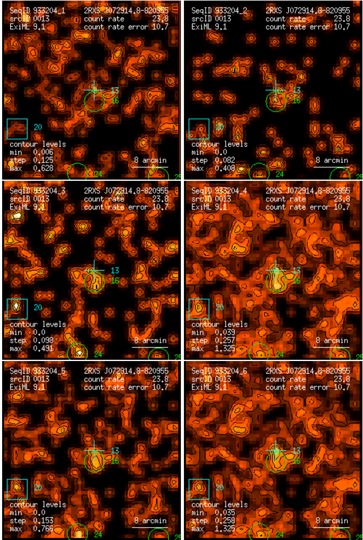
Figure 13: RASS 933204: detection 0013: band rate images, Gaussian filter: (1) PSPC channels 11 – 41, (2) 52 – 90, (3) 91 – 201, (4) 11 – 235, (5) 52 – 201, (6) 11 – 201. Broad band rates in counts/ks. Band rate contour levels in counts/ks/arcmin 2 .
