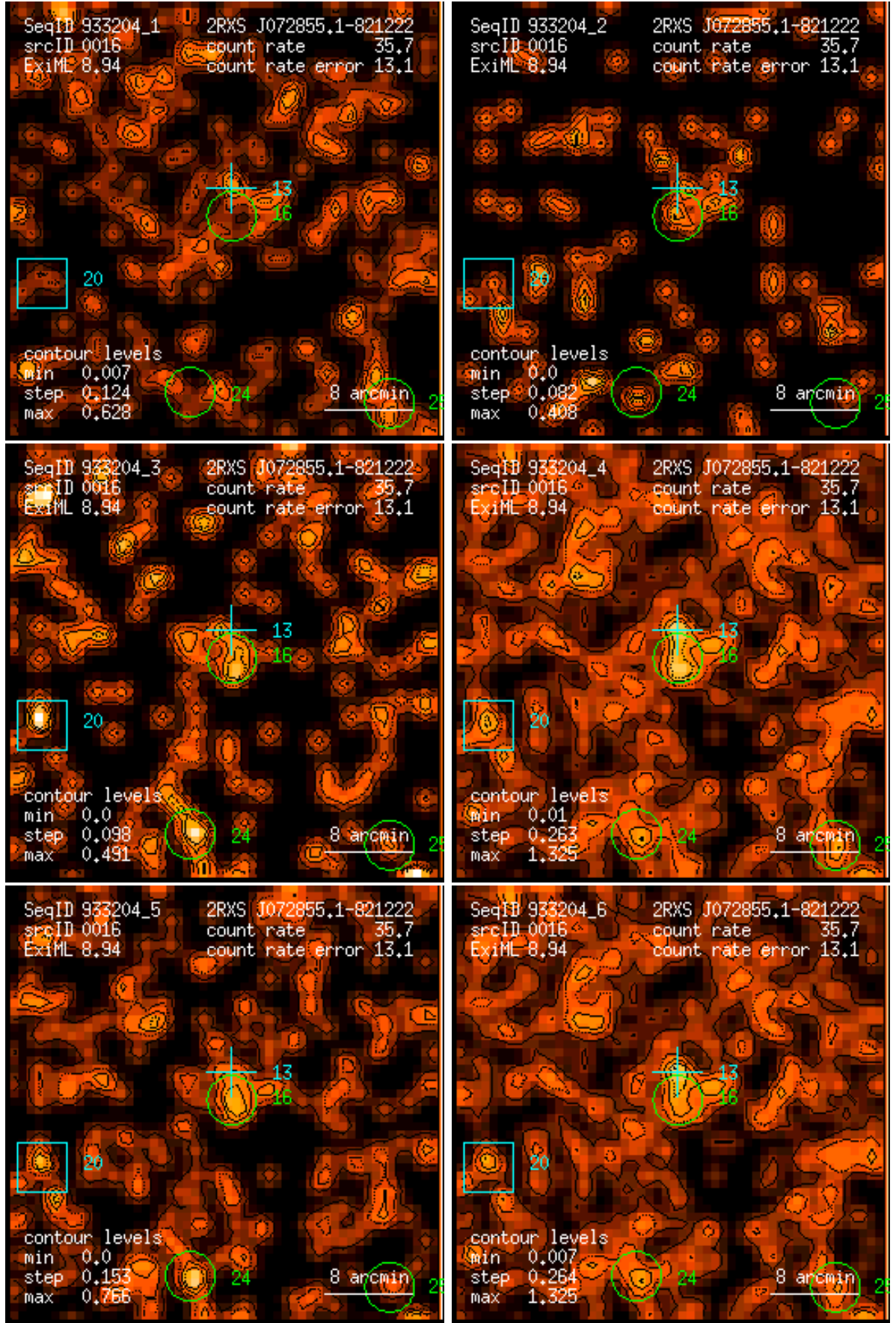
Figure 16: RASS 933204: detection 0016: band rate images, Gaussian filter: (1) PSPC channels 11 – 41, (2) 52 – 90, (3) 91 – 201, (4) 11 – 235, (5) 52 – 201, (6) 11 – 201. Broad band rates in counts/ks. Band rate contour levels in counts/ks/arcmin 2 .
