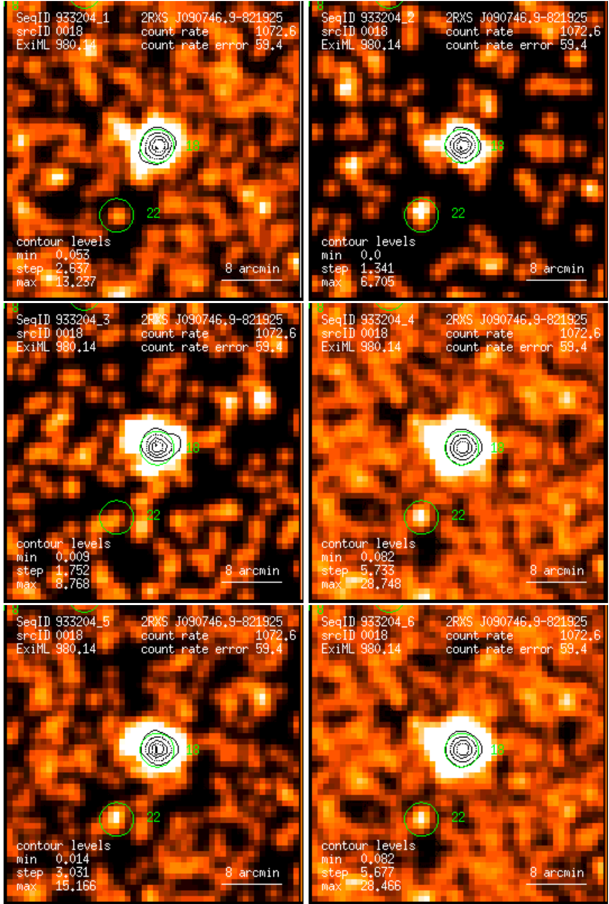
Figure 18: RASS 933204: detection 0018: band rate images, Gaussian filter: (1) PSPC channels 11 – 41, (2) 52 – 90, (3) 91 – 201, (4) 11 – 235, (5) 52 – 201, (6) 11 – 201. Broad band rates in counts/ks. Band rate contour levels in counts/ks/arcmin 2 .
