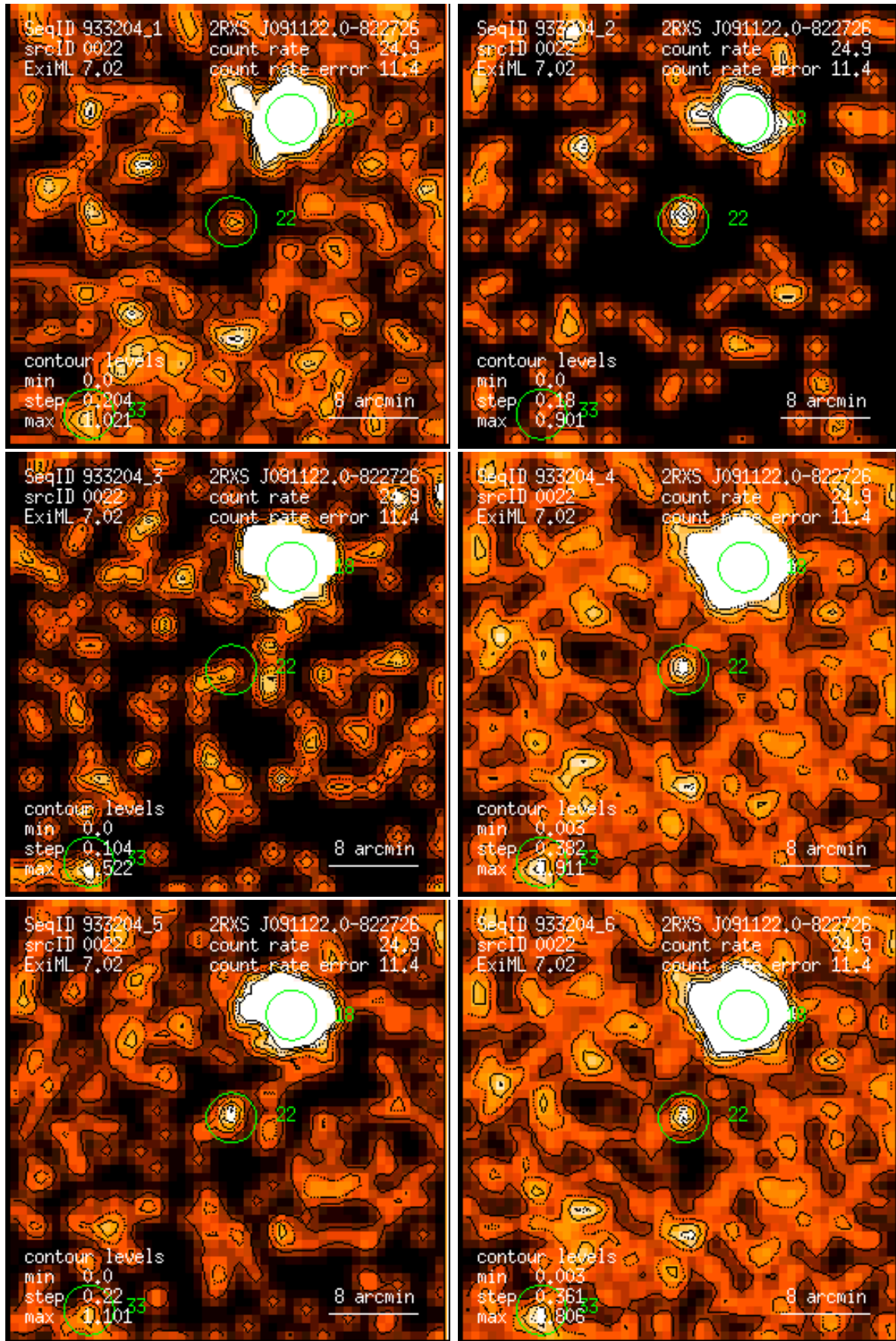
Figure 22: RASS 933204: detection 0022: band rate images, Gaussian filter: (1) PSPC channels 11 – 41, (2) 52 – 90, (3) 91 – 201, (4) 11 – 235, (5) 52 – 201, (6) 11 – 201. Broad band rates in counts/ks. Band rate contour levels in counts/ks/arcmin 2 .
