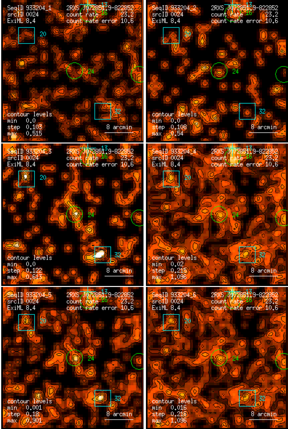
Figure 24: RASS 933204: detection 0024: band rate images, Gaussian filter: (1) PSPC channels 11 – 41, (2) 52 – 90, (3) 91 – 201, (4) 11 – 235, (5) 52 – 201, (6) 11 – 201. Broad band rates in counts/ks. Band rate contour levels in counts/ks/arcmin 2 .
