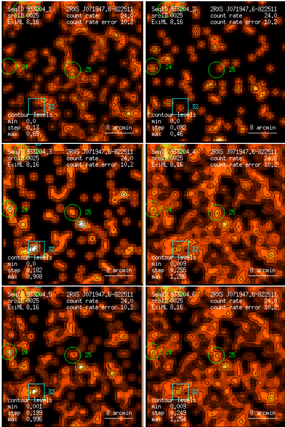
Figure 25: RASS 933204: detection 0025: band rate images, Gaussian filter: (1) PSPC channels 11 – 41, (2) 52 – 90, (3) 91 – 201, (4) 11 – 235, (5) 52 – 201, (6) 11 – 201. Broad band rates in counts/ks. Band rate contour levels in counts/ks/arcmin 2 .
