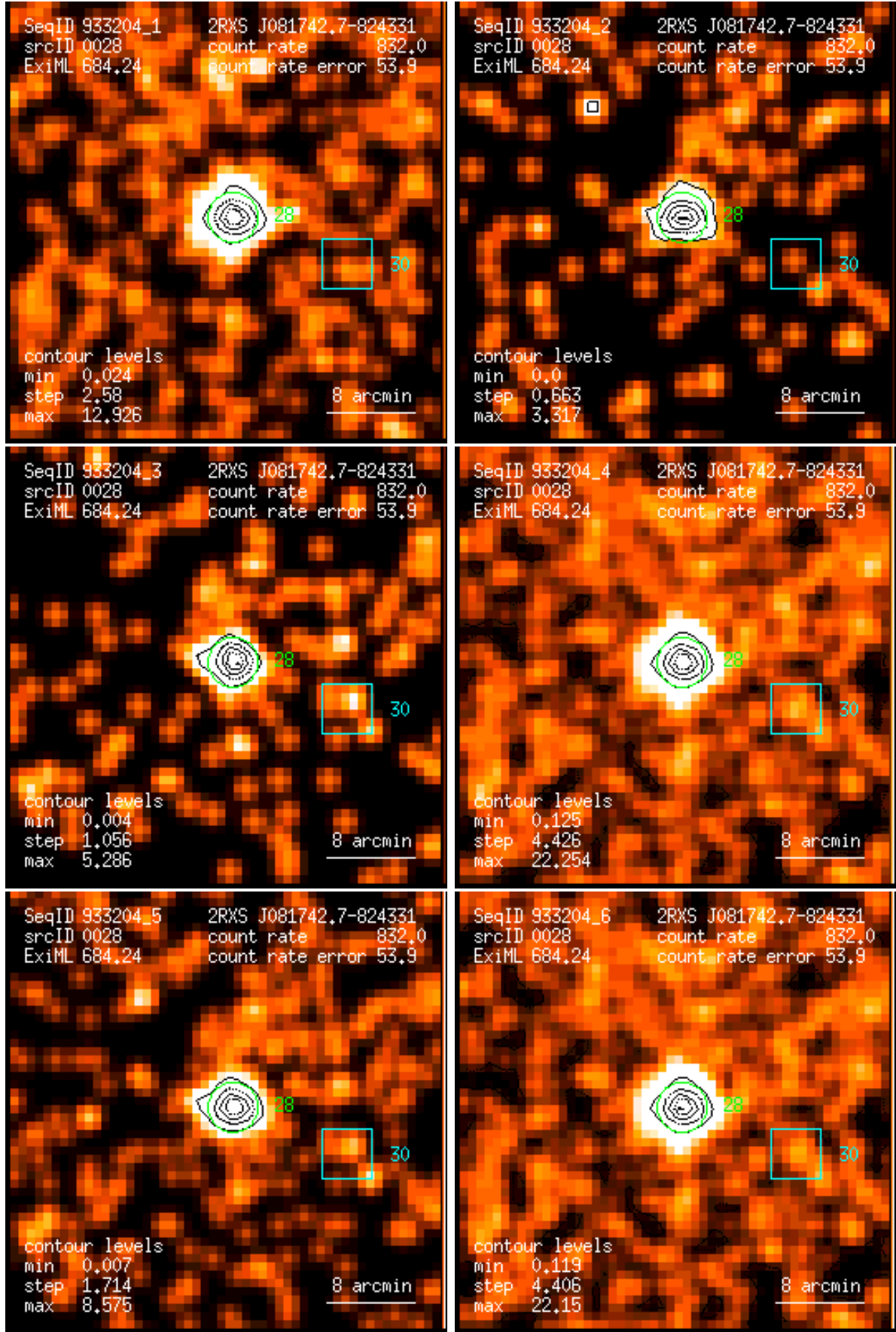
Figure 28: RASS 933204: detection 0028: band rate images, Gaussian filter: (1) PSPC channels 11 – 41, (2) 52 – 90, (3) 91 – 201, (4) 11 – 235, (5) 52 – 201, (6) 11 – 201. Broad band rates in counts/ks. Band rate contour levels in counts/ks/arcmin 2 .
