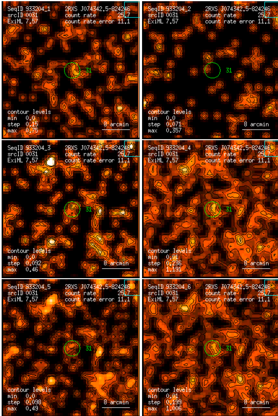
Figure 31: RASS 933204: detection 0031: band rate images, Gaussian filter: (1) PSPC channels 11 – 41, (2) 52 – 90, (3) 91 – 201, (4) 11 – 235, (5) 52 – 201, (6) 11 – 201. Broad band rates in counts/ks. Band rate contour levels in counts/ks/arcmin 2 .
