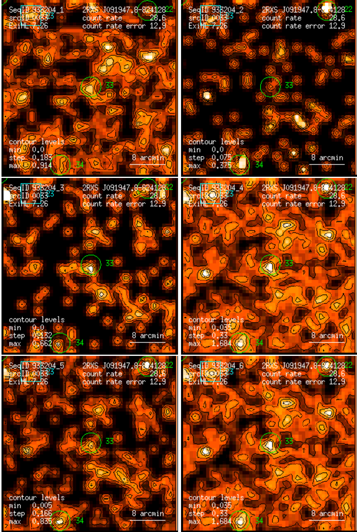
Figure 33: RASS 933204: detection 0033: band rate images, Gaussian filter: (1) PSPC channels 11 – 41, (2) 52 – 90, (3) 91 – 201, (4) 11 – 235, (5) 52 – 201, (6) 11 – 201. Broad band rates in counts/ks. Band rate contour levels in counts/ks/arcmin 2 .
