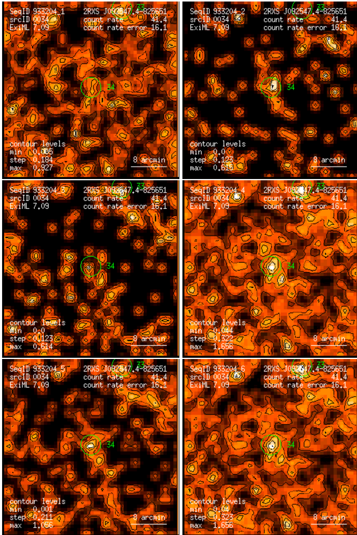
Figure 34: RASS 933204: detection 0034: band rate images, Gaussian filter: (1) PSPC channels 11 – 41, (2) 52 – 90, (3) 91 – 201, (4) 11 – 235, (5) 52 – 201, (6) 11 – 201. Broad band rates in counts/ks. Band rate contour levels in counts/ks/arcmin 2 .
