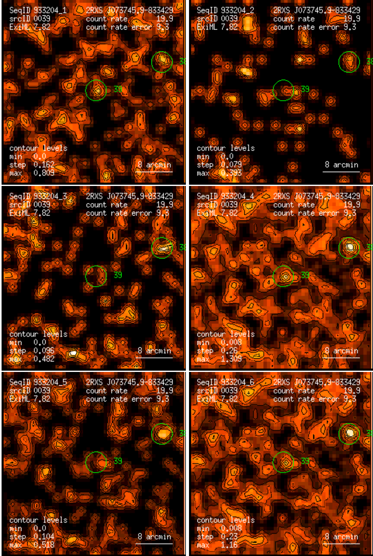
Figure 39: RASS 933204: detection 0039: band rate images, Gaussian filter: (1) PSPC channels 11 – 41, (2) 52 – 90, (3) 91 – 201, (4) 11 – 235, (5) 52 – 201, (6) 11 – 201. Broad band rates in counts/ks. Band rate contour levels in counts/ks/arcmin 2 .
