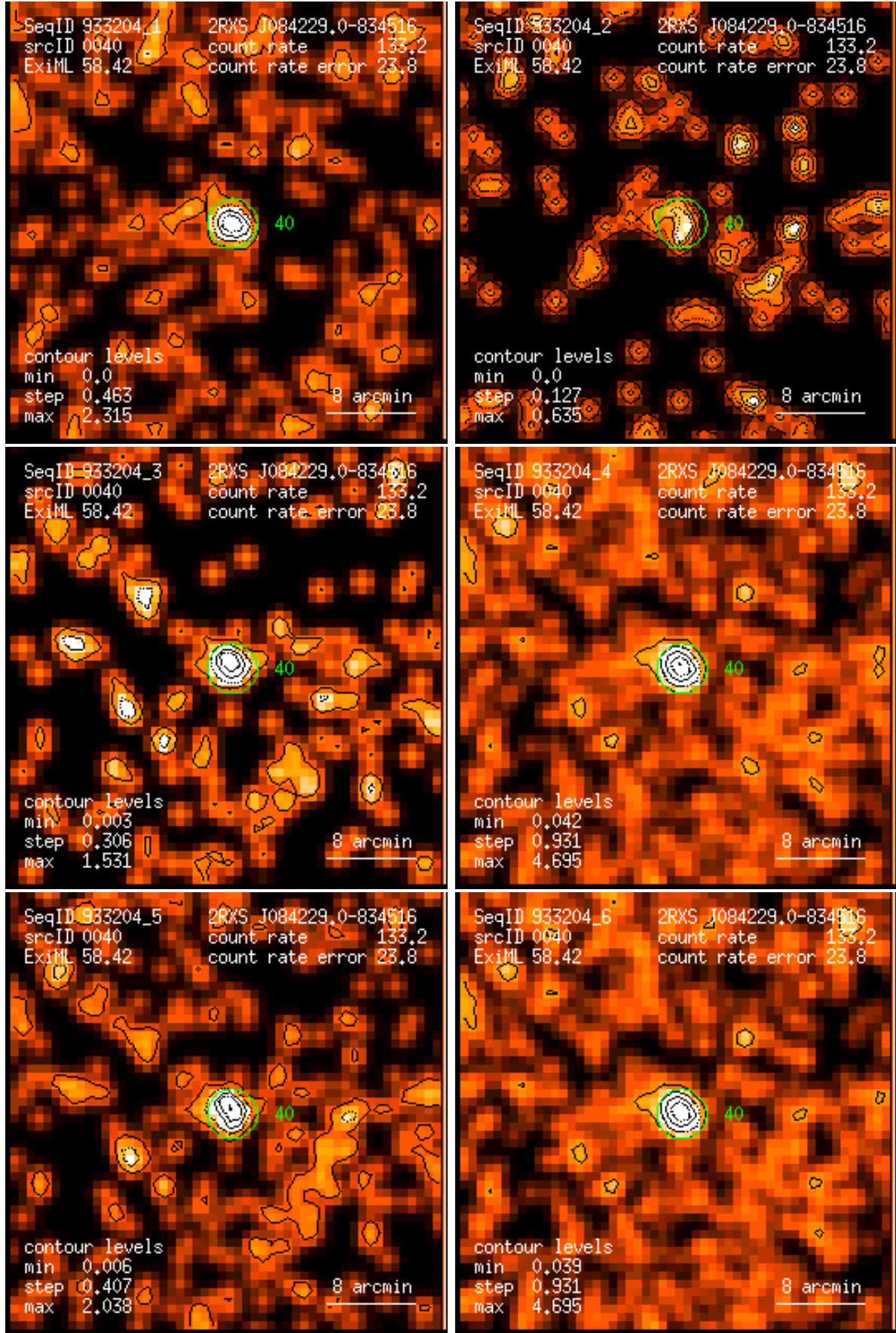
Figure 40: RASS 933204: detection 0040: band rate images, Gaussian filter: (1) PSPC channels 11 – 41, (2) 52 – 90, (3) 91 – 201, (4) 11 – 235, (5) 52 – 201, (6) 11 – 201. Broad band rates in counts/ks. Band rate contour levels in counts/ks/arcmin 2 .
