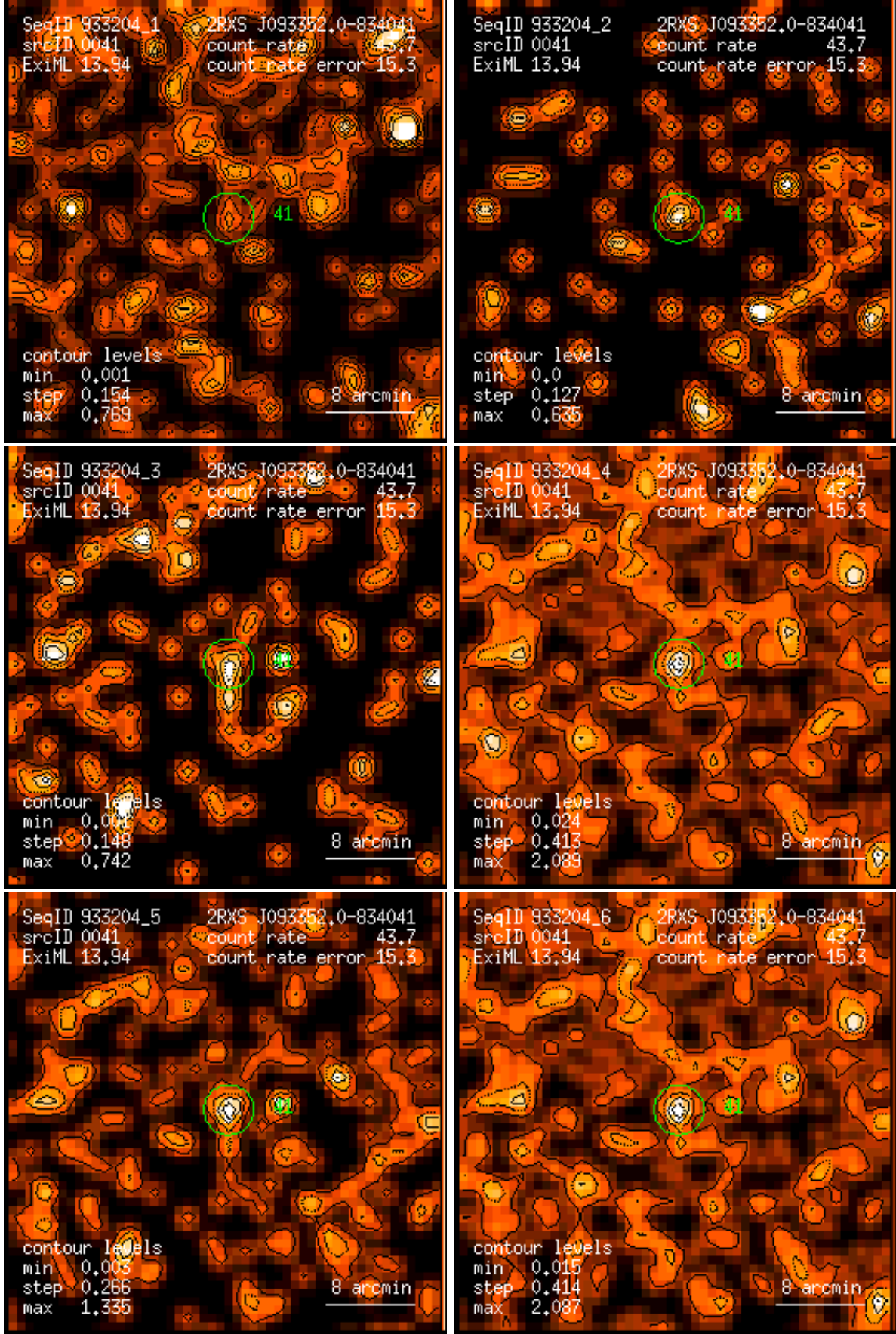
Figure 41: RASS 933204: detection 0041: band rate images, Gaussian filter: (1) PSPC channels 11 – 41, (2) 52 – 90, (3) 91 – 201, (4) 11 – 235, (5) 52 – 201, (6) 11 – 201. Broad band rates in counts/ks. Band rate contour levels in counts/ks/arcmin 2 .
