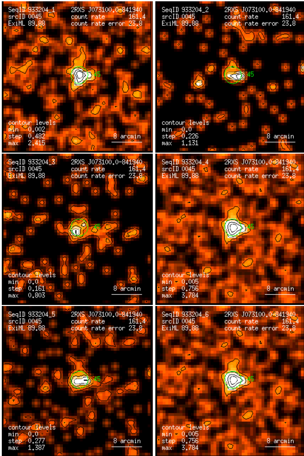
Figure 45: RASS 933204: detection 0045: band rate images, Gaussian filter: (1) PSPC channels 11 – 41, (2) 52 – 90, (3) 91 – 201, (4) 11 – 235, (5) 52 – 201, (6) 11 – 201. Broad band rates in counts/ks. Band rate contour levels in counts/ks/arcmin 2 .
