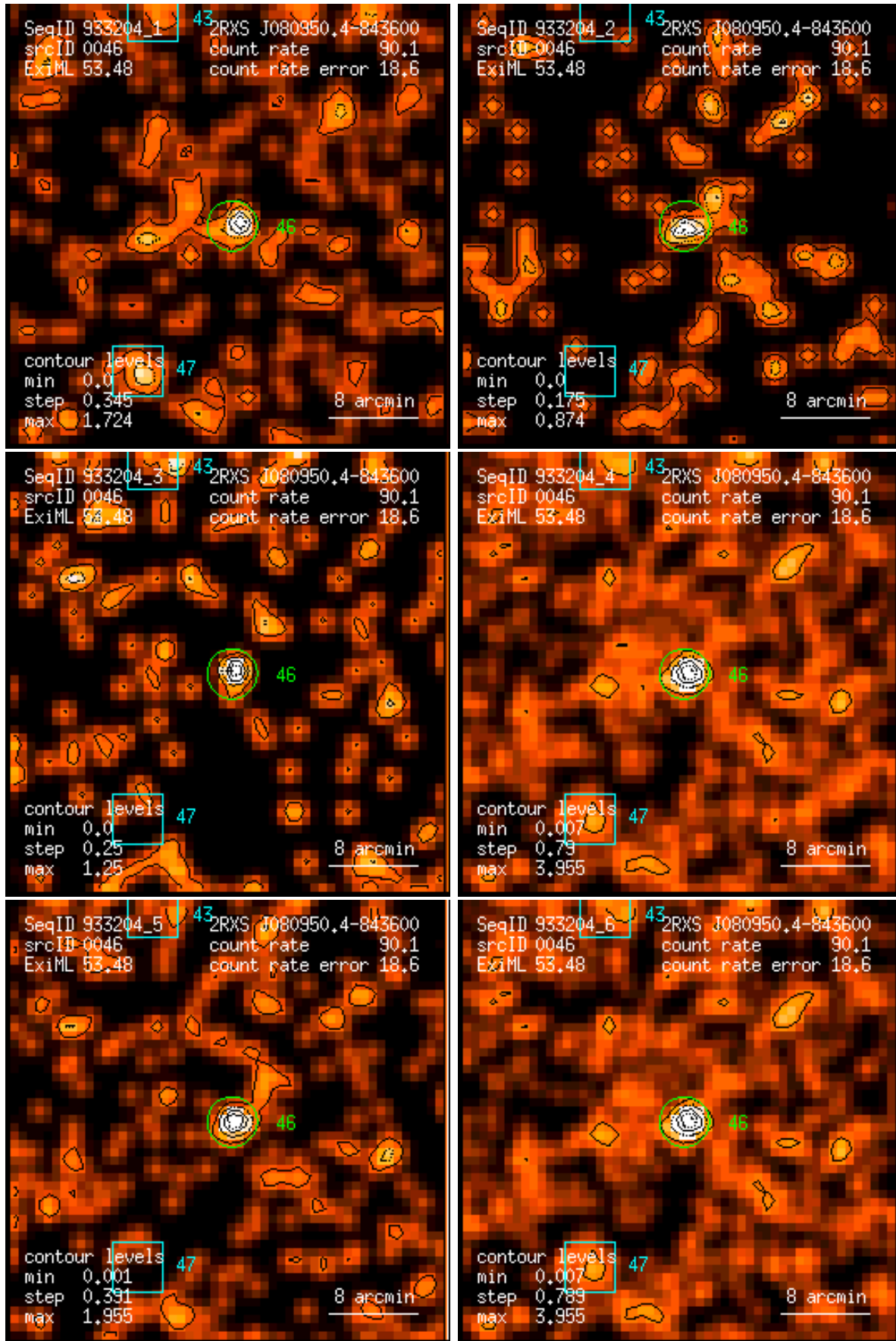
Figure 46: RASS 933204: detection 0046: band rate images, Gaussian filter: (1) PSPC channels 11 – 41, (2) 52 – 90, (3) 91 – 201, (4) 11 – 235, (5) 52 – 201, (6) 11 – 201. Broad band rates in counts/ks. Band rate contour levels in counts/ks/arcmin 2 .
