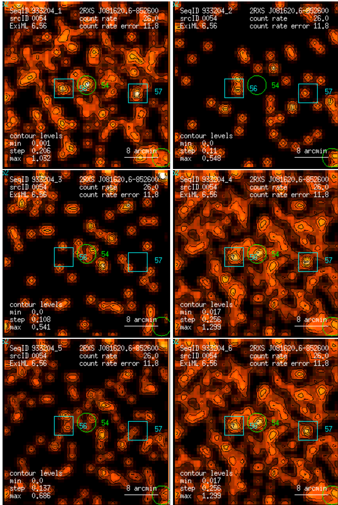
Figure 54: RASS 933204: detection 0054: band rate images, Gaussian filter: (1) PSPC channels 11 – 41, (2) 52 – 90, (3) 91 – 201, (4) 11 – 235, (5) 52 – 201, (6) 11 – 201. Broad band rates in counts/ks. Band rate contour levels in counts/ks/arcmin 2 .
