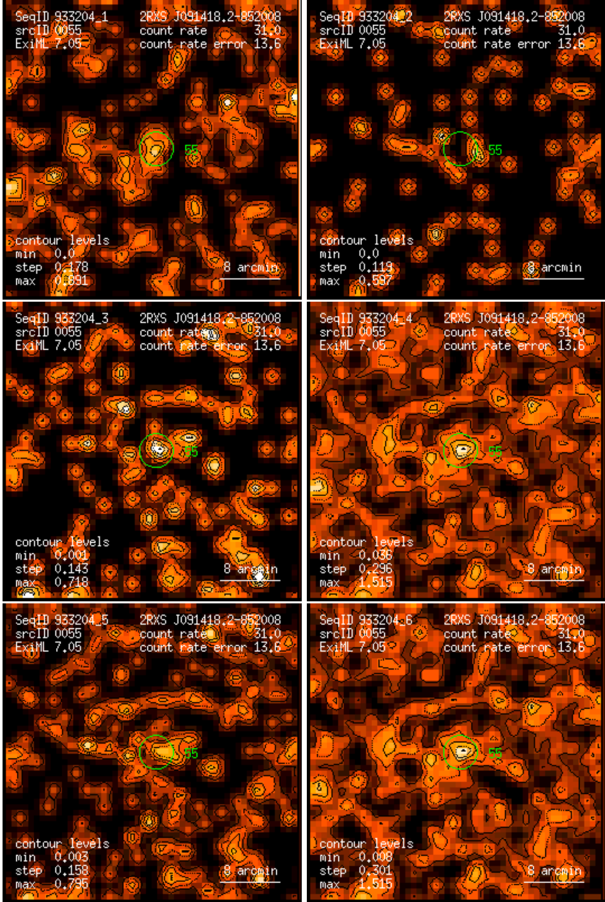
Figure 55: RASS 933204: detection 0055: band rate images, Gaussian filter: (1) PSPC channels 11 – 41, (2) 52 – 90, (3) 91 – 201, (4) 11 – 235, (5) 52 – 201, (6) 11 – 201. Broad band rates in counts/ks. Band rate contour levels in counts/ks/arcmin 2 .
