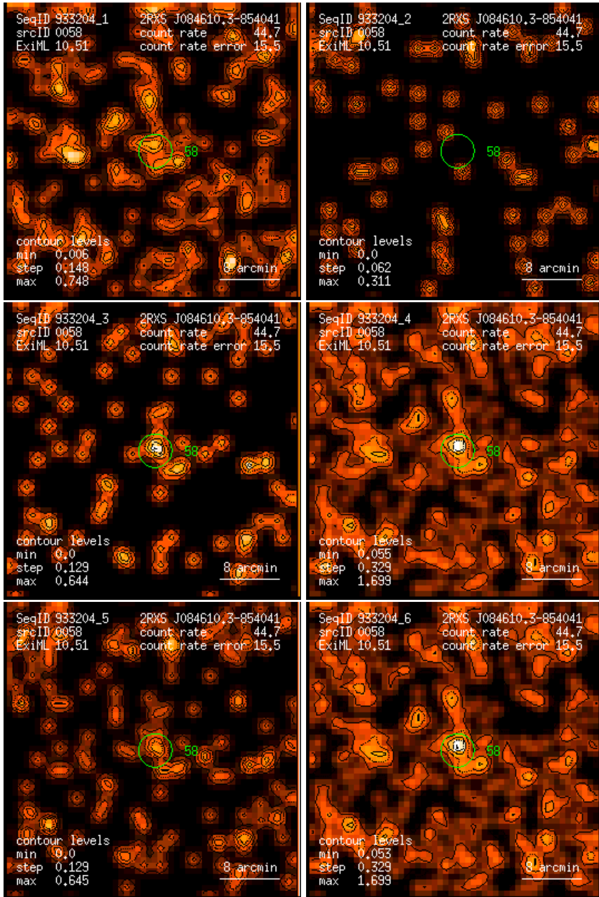
Figure 58: RASS 933204: detection 0058: band rate images, Gaussian filter: (1) PSPC channels 11 – 41, (2) 52 – 90, (3) 91 – 201, (4) 11 – 235, (5) 52 – 201, (6) 11 – 201. Broad band rates in counts/ks. Band rate contour levels in counts/ks/arcmin 2 .
