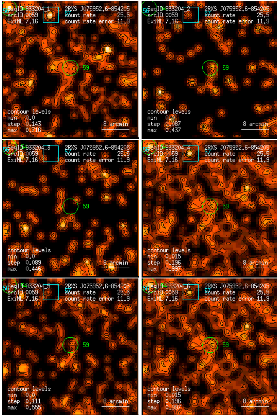
Figure 59: RASS 933204: detection 0059: band rate images, Gaussian filter: (1) PSPC channels 11 – 41, (2) 52 – 90, (3) 91 – 201, (4) 11 – 235, (5) 52 – 201, (6) 11 – 201. Broad band rates in counts/ks. Band rate contour levels in counts/ks/arcmin 2 .
