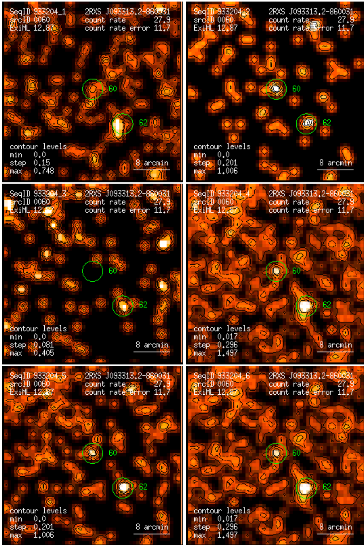
Figure 60: RASS 933204: detection 0060: band rate images, Gaussian filter: (1) PSPC channels 11 – 41, (2) 52 – 90, (3) 91 – 201, (4) 11 – 235, (5) 52 – 201, (6) 11 – 201. Broad band rates in counts/ks. Band rate contour levels in counts/ks/arcmin 2 .
