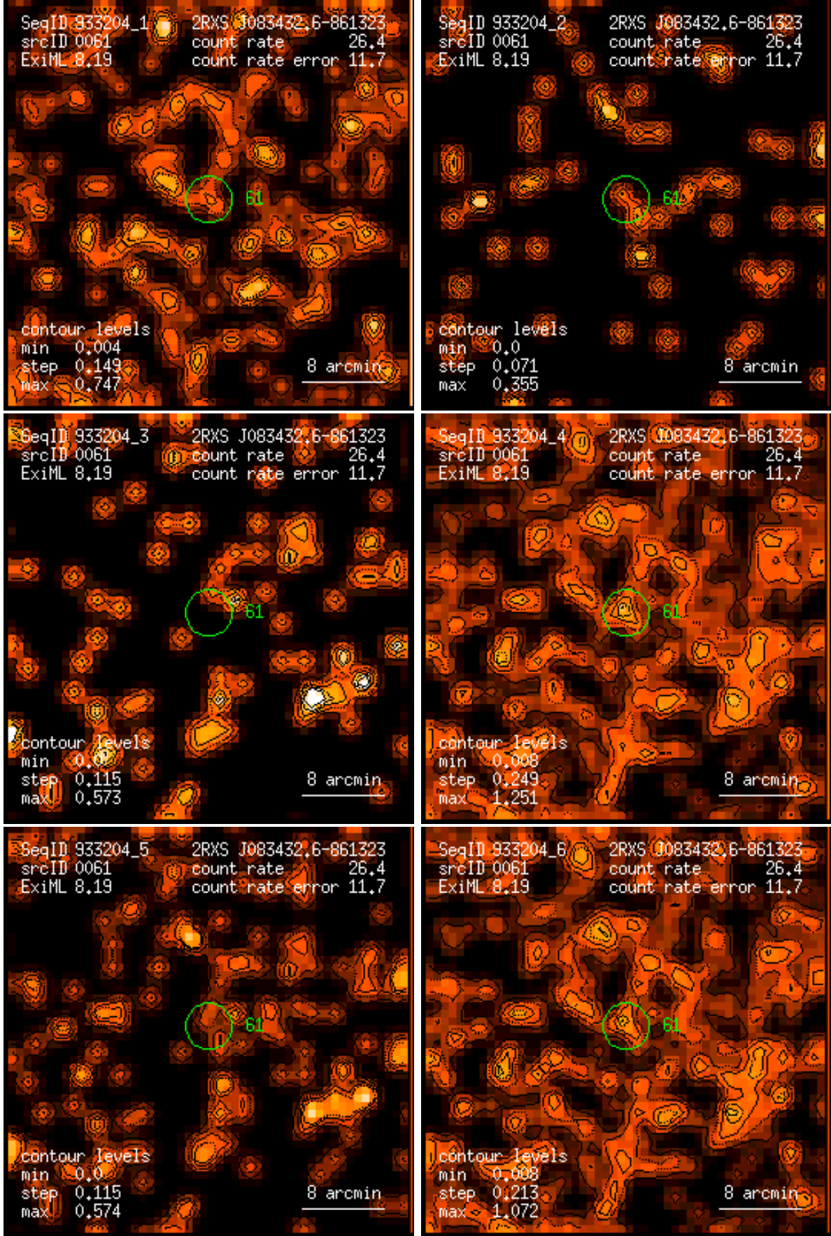
Figure 61: RASS 933204: detection 0061: band rate images, Gaussian filter: (1) PSPC channels 11 – 41, (2) 52 – 90, (3) 91 – 201, (4) 11 – 235, (5) 52 – 201, (6) 11 – 201. Broad band rates in counts/ks. Band rate contour levels in counts/ks/arcmin 2 .
