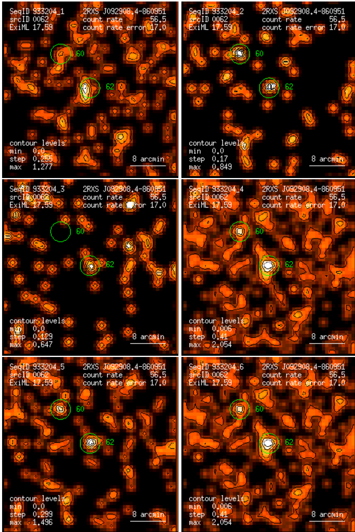
Figure 62: RASS 933204: detection 0062: band rate images, Gaussian filter: (1) PSPC channels 11 – 41, (2) 52 – 90, (3) 91 – 201, (4) 11 – 235, (5) 52 – 201, (6) 11 – 201. Broad band rates in counts/ks. Band rate contour levels in counts/ks/arcmin 2 .
