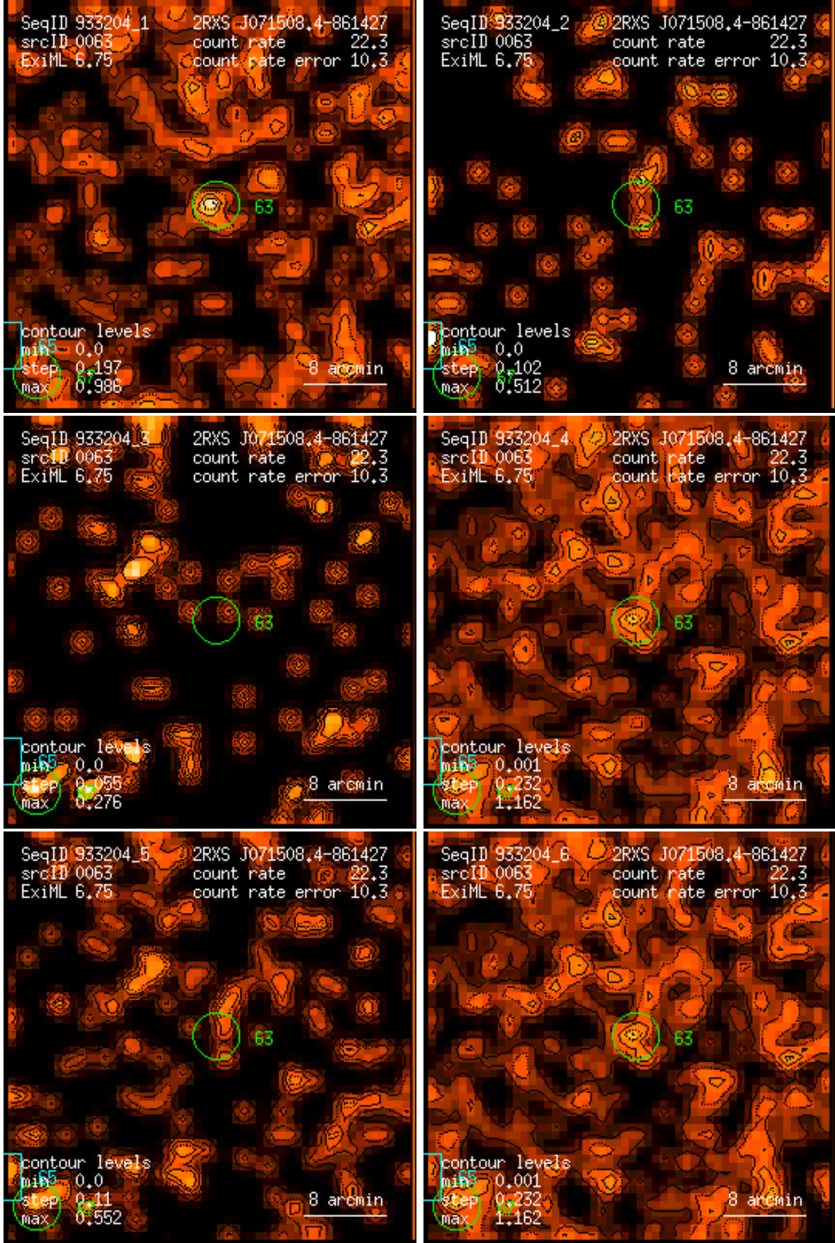
Figure 63: RASS 933204: detection 0063: band rate images, Gaussian filter: (1) PSPC channels 11 – 41, (2) 52 – 90, (3) 91 – 201, (4) 11 – 235, (5) 52 – 201, (6) 11 – 201. Broad band rates in counts/ks. Band rate contour levels in counts/ks/arcmin 2 .
