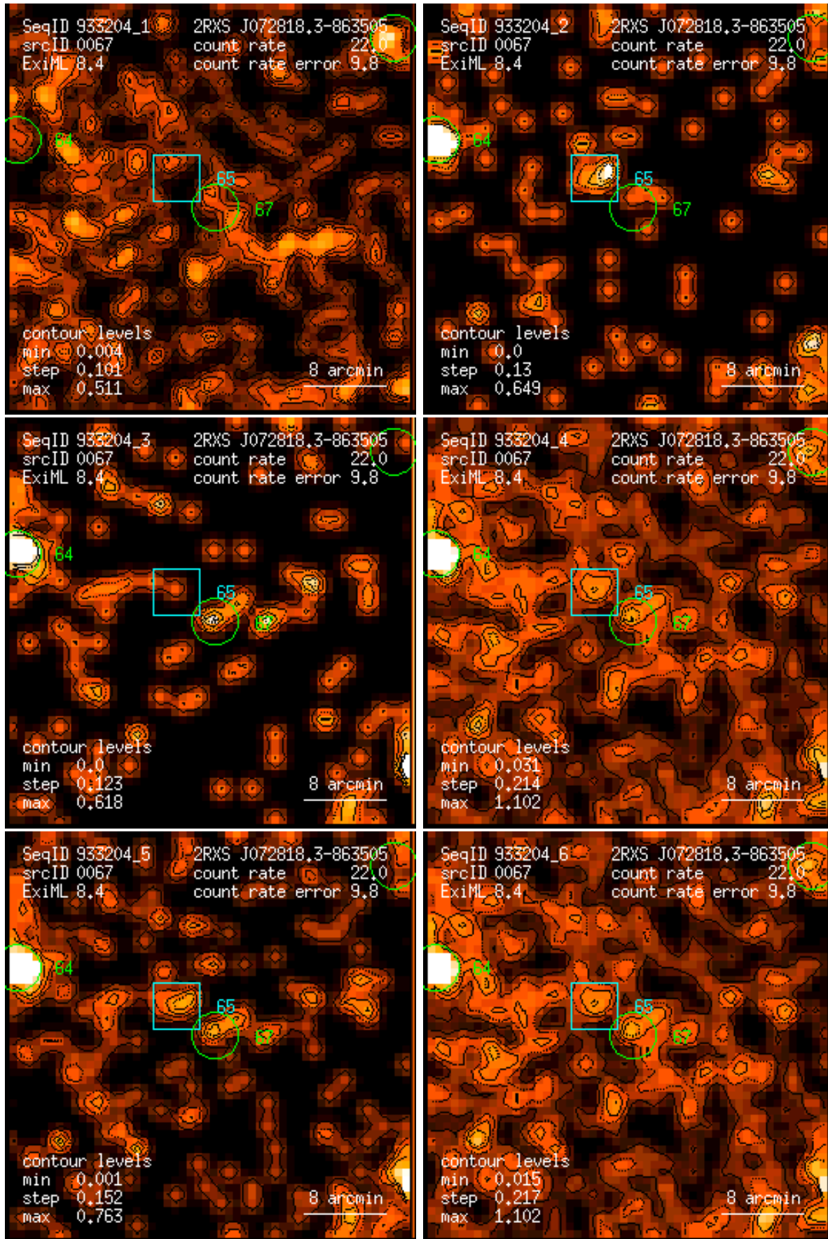
Figure 67: RASS 933204: detection 0067: band rate images, Gaussian filter: (1) PSPC channels 11 – 41, (2) 52 – 90, (3) 91 – 201, (4) 11 – 235, (5) 52 – 201, (6) 11 – 201. Broad band rates in counts/ks. Band rate contour levels in counts/ks/arcmin 2 .
