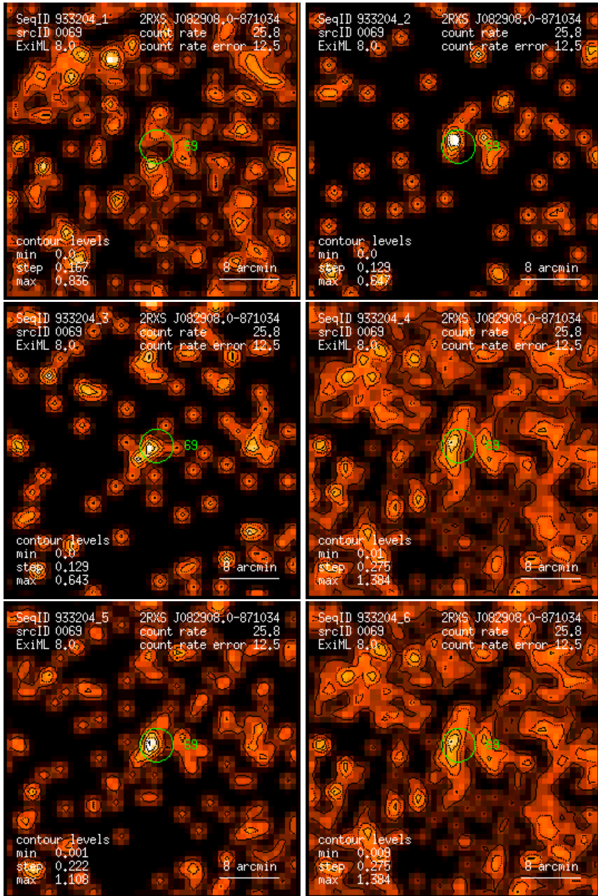
Figure 69: RASS 933204: detection 0069: band rate images, Gaussian filter: (1) PSPC channels 11 – 41, (2) 52 – 90, (3) 91 – 201, (4) 11 – 235, (5) 52 – 201, (6) 11 – 201. Broad band rates in counts/ks. Band rate contour levels in counts/ks/arcmin 2 .
