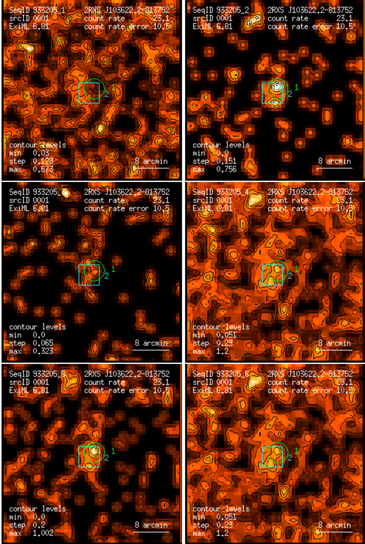
Figure 1: RASS 933205: detection 0001: band rate images, Gaussian filter: (1) PSPC channels 11 – 41, (2) 52 – 90, (3) 91 – 201, (4) 11 – 235, (5) 52 – 201, (6) 11 – 201. Broad band rates in counts/ks. Band rate contour levels in counts/ks/arcmin 2 .
