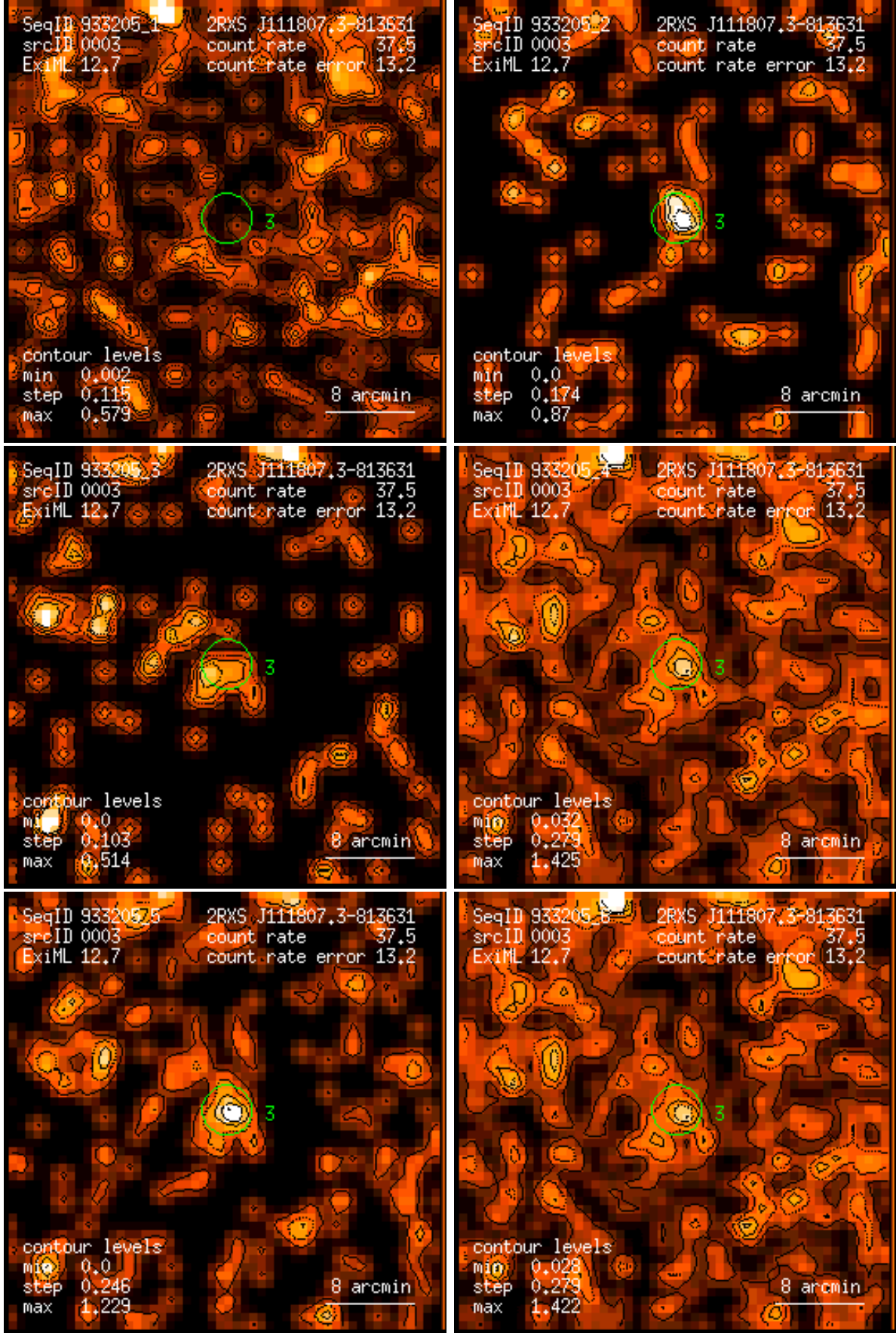
Figure 3: RASS 933205: detection 0003: band rate images, Gaussian filter: (1) PSPC channels 11 – 41, (2) 52 – 90, (3) 91 – 201, (4) 11 – 235, (5) 52 – 201, (6) 11 – 201. Broad band rates in counts/ks. Band rate contour levels in counts/ks/arcmin 2 .
