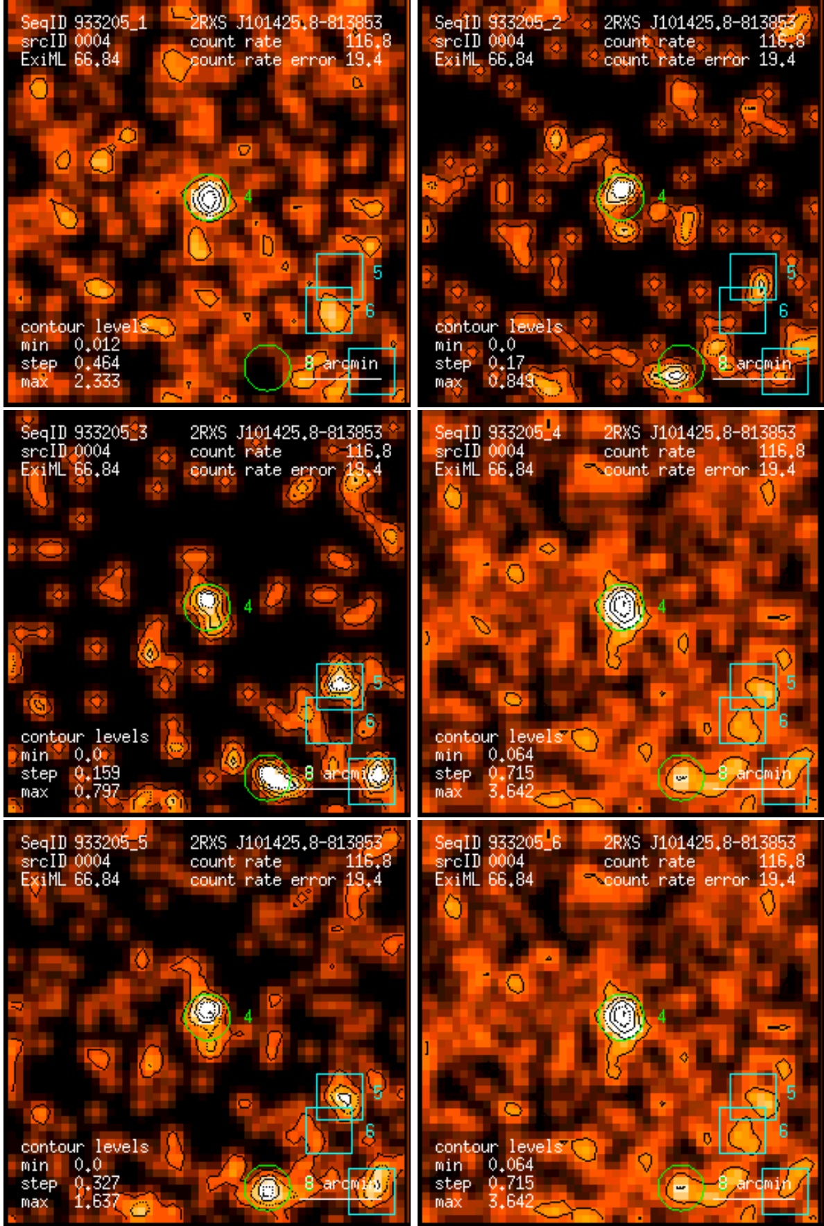
Figure 4: RASS 933205: detection 0004: band rate images, Gaussian filter: (1) PSPC channels 11 – 41, (2) 52 – 90, (3) 91 – 201, (4) 11 – 235, (5) 52 – 201, (6) 11 – 201. Broad band rates in counts/ks. Band rate contour levels in counts/ks/arcmin 2 .
