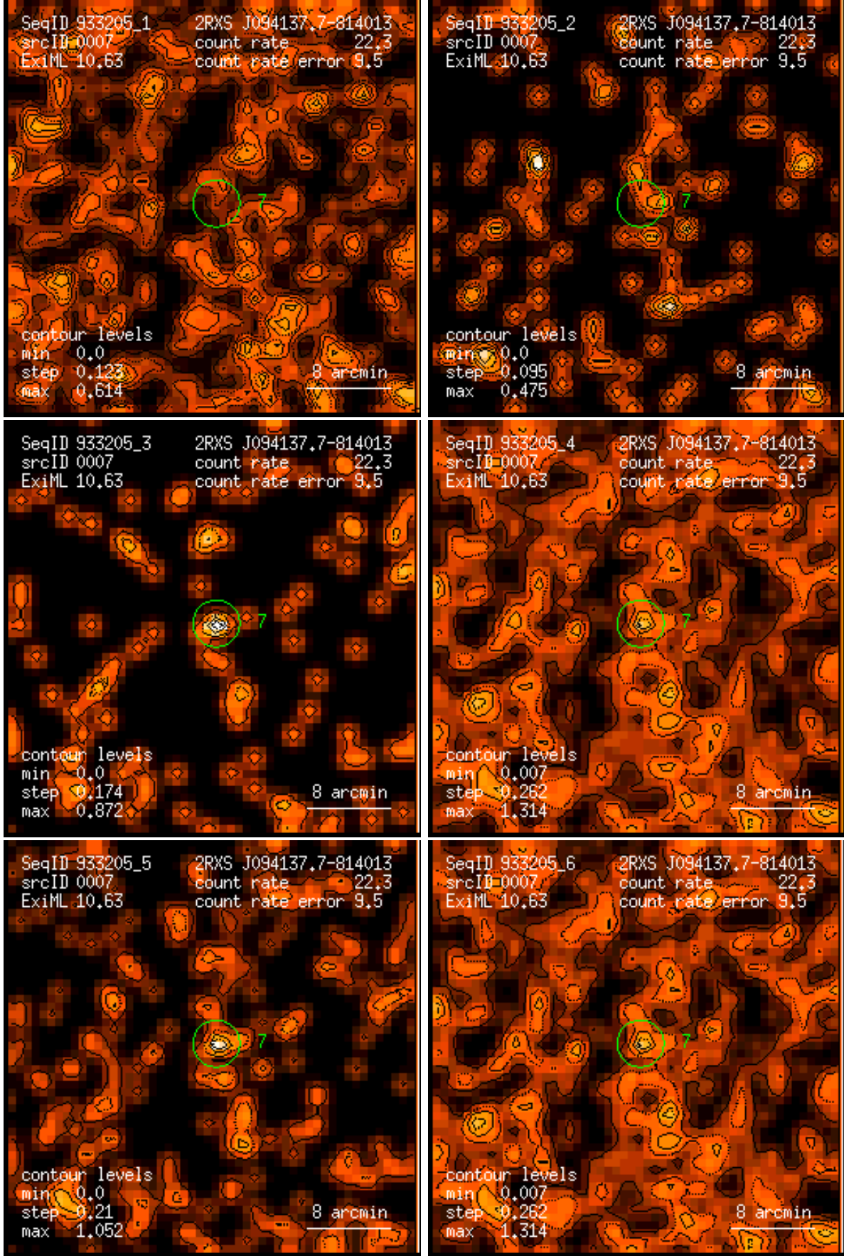
Figure 7: RASS 933205: detection 0007: band rate images, Gaussian filter: (1) PSPC channels 11 – 41, (2) 52 – 90, (3) 91 – 201, (4) 11 – 235, (5) 52 – 201, (6) 11 – 201. Broad band rates in counts/ks. Band rate contour levels in counts/ks/arcmin 2 .
