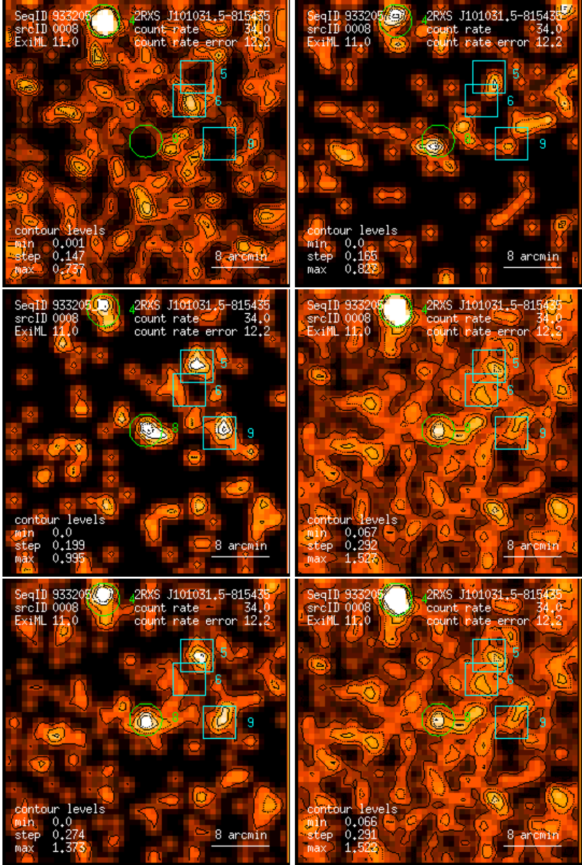
Figure 8: RASS 933205: detection 0008: band rate images, Gaussian filter: (1) PSPC channels 11 – 41, (2) 52 – 90, (3) 91 – 201, (4) 11 – 235, (5) 52 – 201, (6) 11 – 201. Broad band rates in counts/ks. Band rate contour levels in counts/ks/arcmin 2 .
