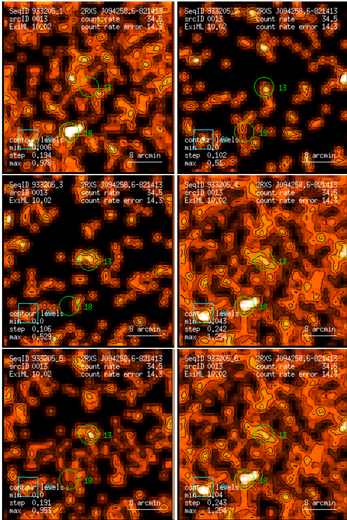
Figure 13: RASS 933205: detection 0013: band rate images, Gaussian filter: (1) PSPC channels 11 – 41, (2) 52 – 90, (3) 91 – 201, (4) 11 – 235, (5) 52 – 201, (6) 11 – 201. Broad band rates in counts/ks. Band rate contour levels in counts/ks/arcmin 2 .
