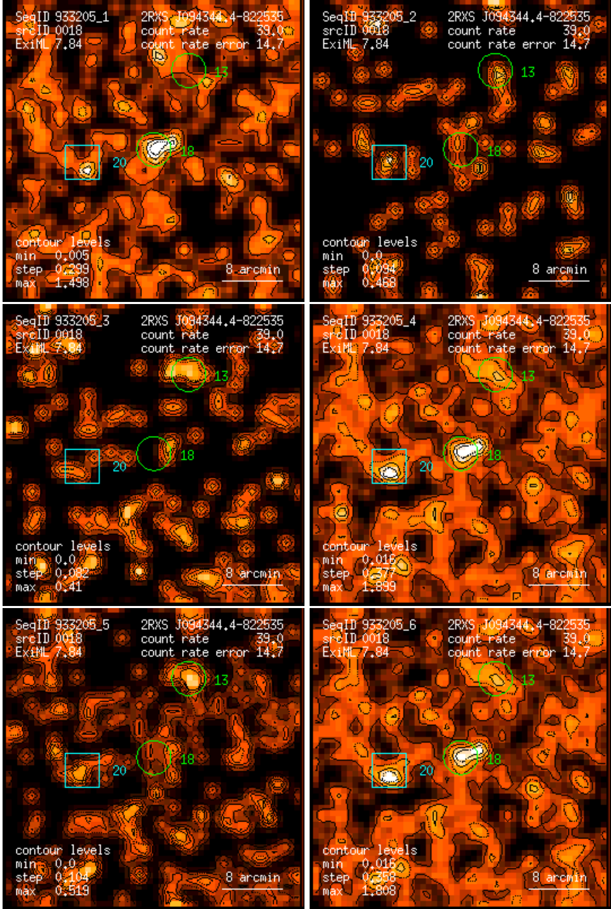
Figure 18: RASS 933205: detection 0018: band rate images, Gaussian filter: (1) PSPC channels 11 – 41, (2) 52 – 90, (3) 91 – 201, (4) 11 – 235, (5) 52 – 201, (6) 11 – 201. Broad band rates in counts/ks. Band rate contour levels in counts/ks/arcmin 2 .
