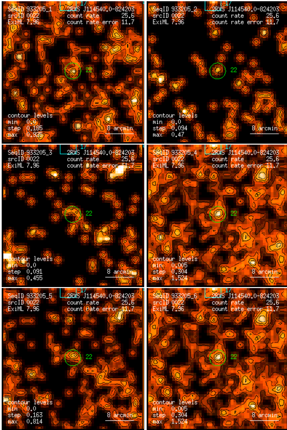
Figure 22: RASS 933205: detection 0022: band rate images, Gaussian filter: (1) PSPC channels 11 – 41, (2) 52 – 90, (3) 91 – 201, (4) 11 – 235, (5) 52 – 201, (6) 11 – 201. Broad band rates in counts/ks. Band rate contour levels in counts/ks/arcmin 2 .
