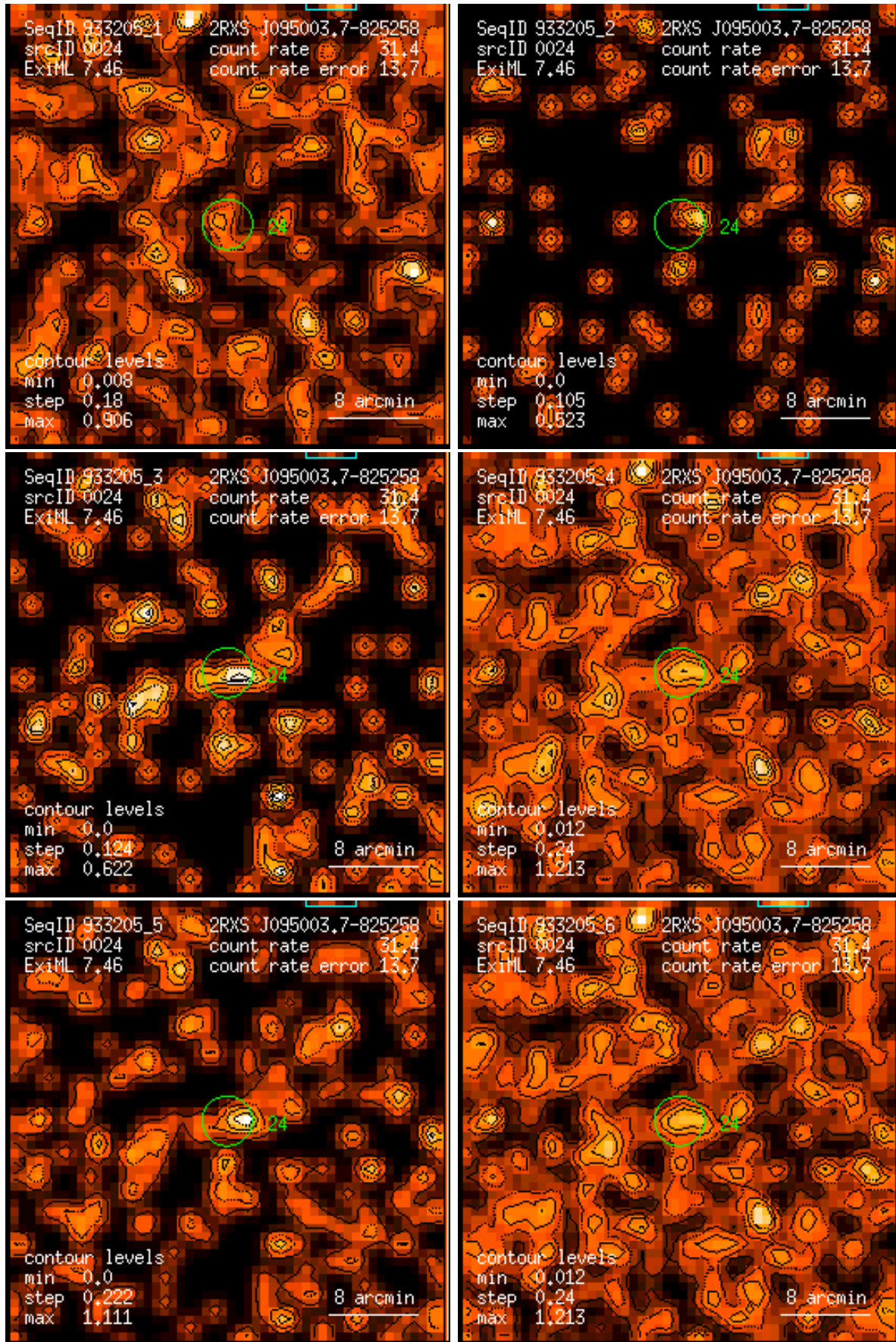
Figure 24: RASS 933205: detection 0024: band rate images, Gaussian filter: (1) PSPC channels 11 – 41, (2) 52 – 90, (3) 91 – 201, (4) 11 – 235, (5) 52 – 201, (6) 11 – 201. Broad band rates in counts/ks. Band rate contour levels in counts/ks/arcmin 2 .
