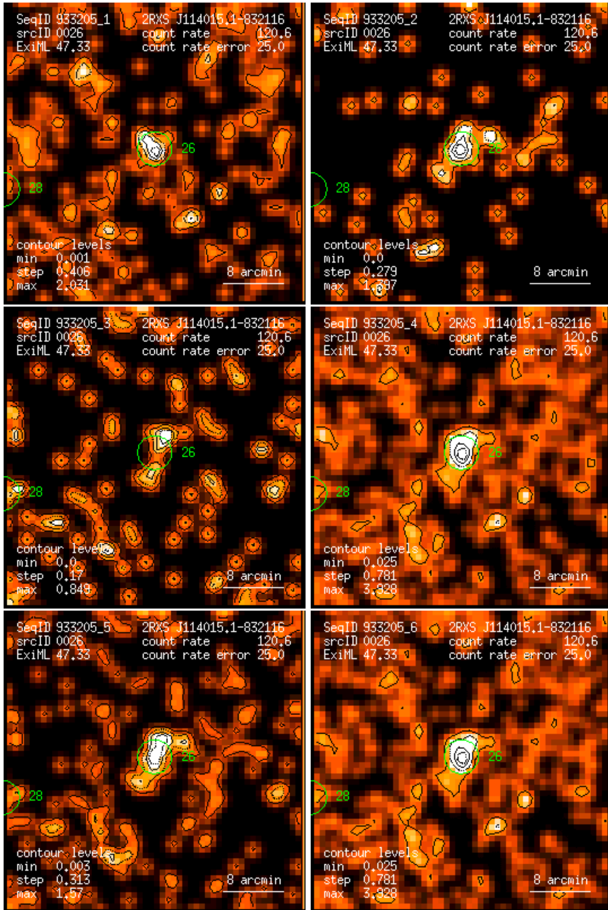
Figure 26: RASS 933205: detection 0026: band rate images, Gaussian filter: (1) PSPC channels 11 – 41, (2) 52 – 90, (3) 91 – 201, (4) 11 – 235, (5) 52 – 201, (6) 11 – 201. Broad band rates in counts/ks. Band rate contour levels in counts/ks/arcmin 2 .
