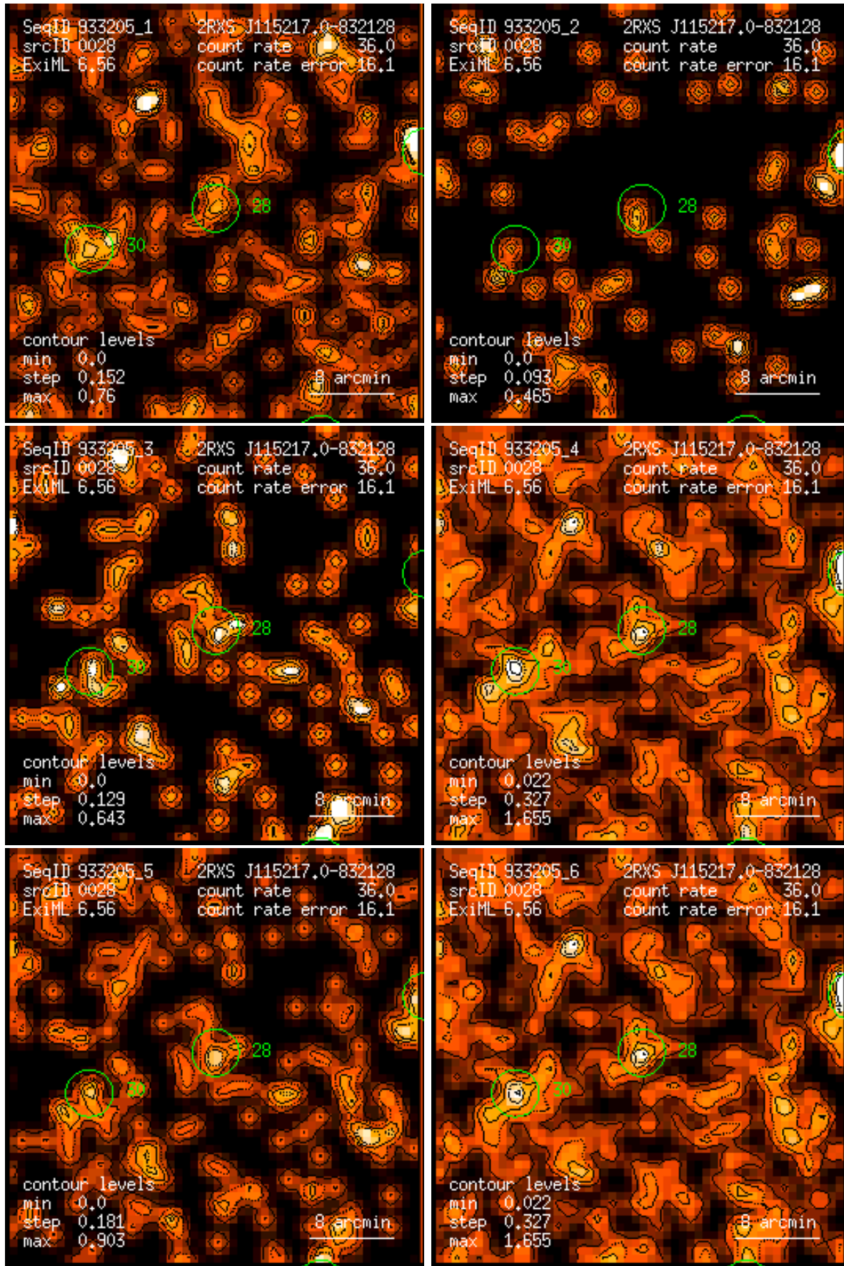
Figure 28: RASS 933205: detection 0028: band rate images, Gaussian filter: (1) PSPC channels 11 – 41, (2) 52 – 90, (3) 91 – 201, (4) 11 – 235, (5) 52 – 201, (6) 11 – 201. Broad band rates in counts/ks. Band rate contour levels in counts/ks/arcmin 2 .
