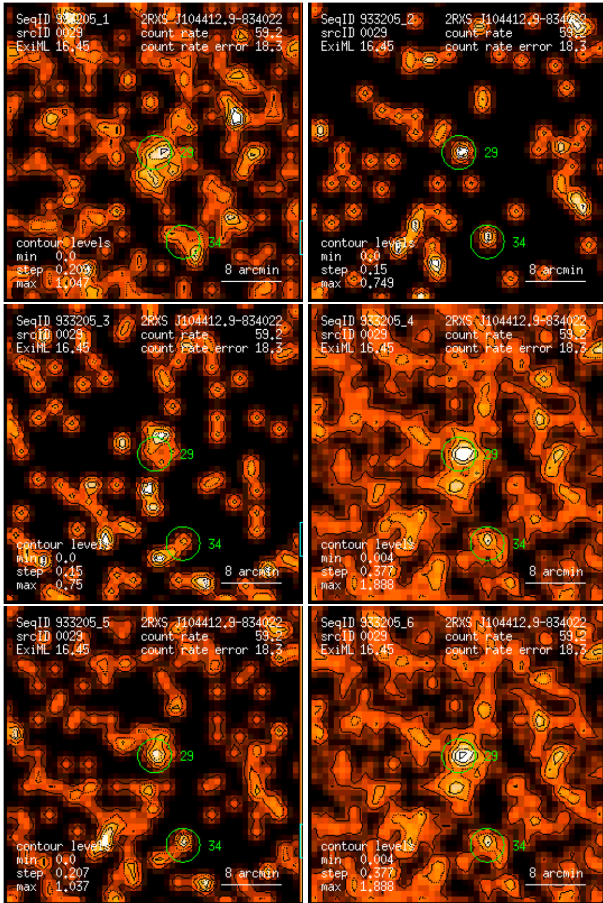
Figure 29: RASS 933205: detection 0029: band rate images, Gaussian filter: (1) PSPC channels 11 – 41, (2) 52 – 90, (3) 91 – 201, (4) 11 – 235, (5) 52 – 201, (6) 11 – 201. Broad band rates in counts/ks. Band rate contour levels in counts/ks/arcmin 2 .
