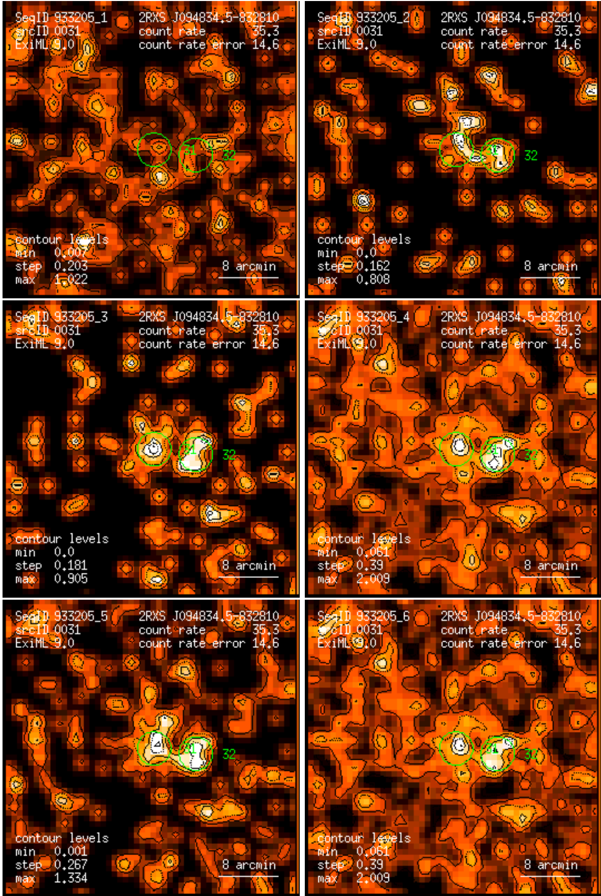
Figure 31: RASS 933205: detection 0031: band rate images, Gaussian filter: (1) PSPC channels 11 – 41, (2) 52 – 90, (3) 91 – 201, (4) 11 – 235, (5) 52 – 201, (6) 11 – 201. Broad band rates in counts/ks. Band rate contour levels in counts/ks/arcmin 2 .
