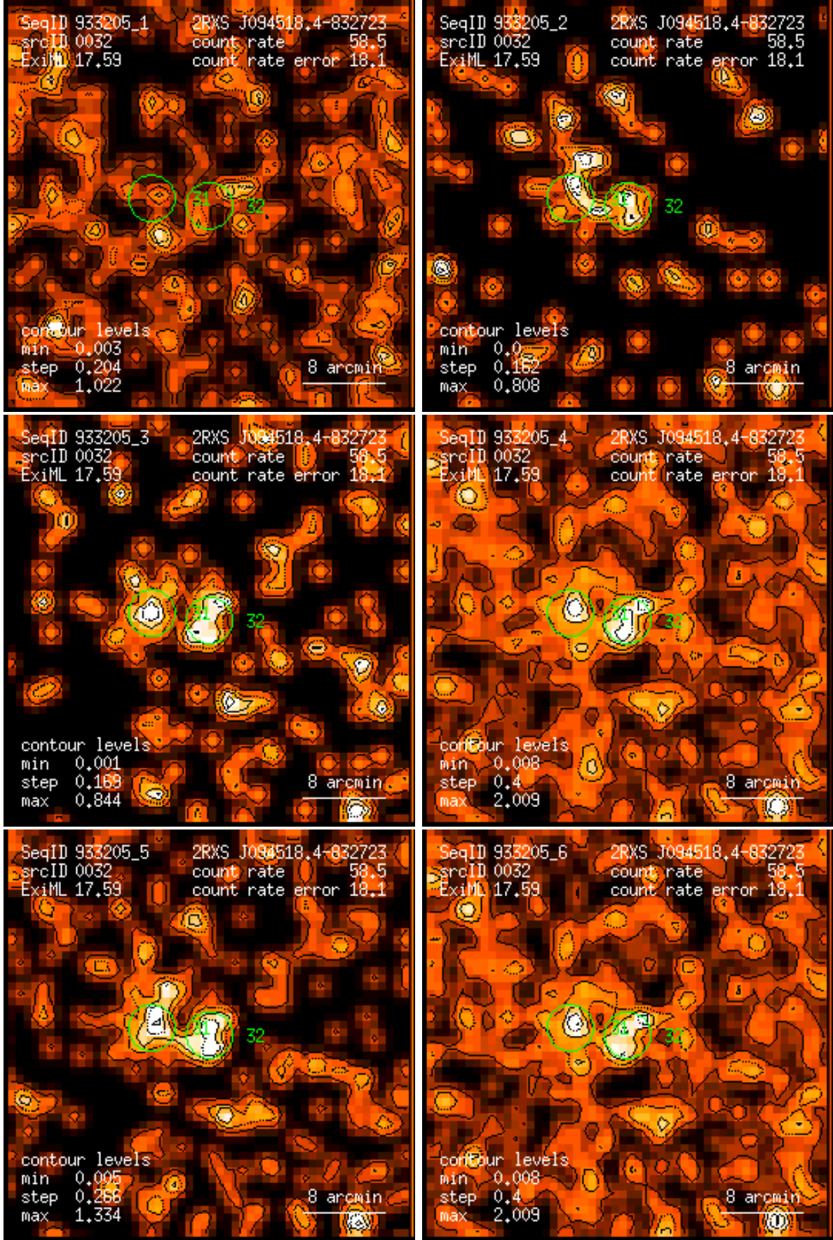
Figure 32: RASS 933205: detection 0032: band rate images, Gaussian filter: (1) PSPC channels 11 – 41, (2) 52 – 90, (3) 91 – 201, (4) 11 – 235, (5) 52 – 201, (6) 11 – 201. Broad band rates in counts/ks. Band rate contour levels in counts/ks/arcmin 2 .
