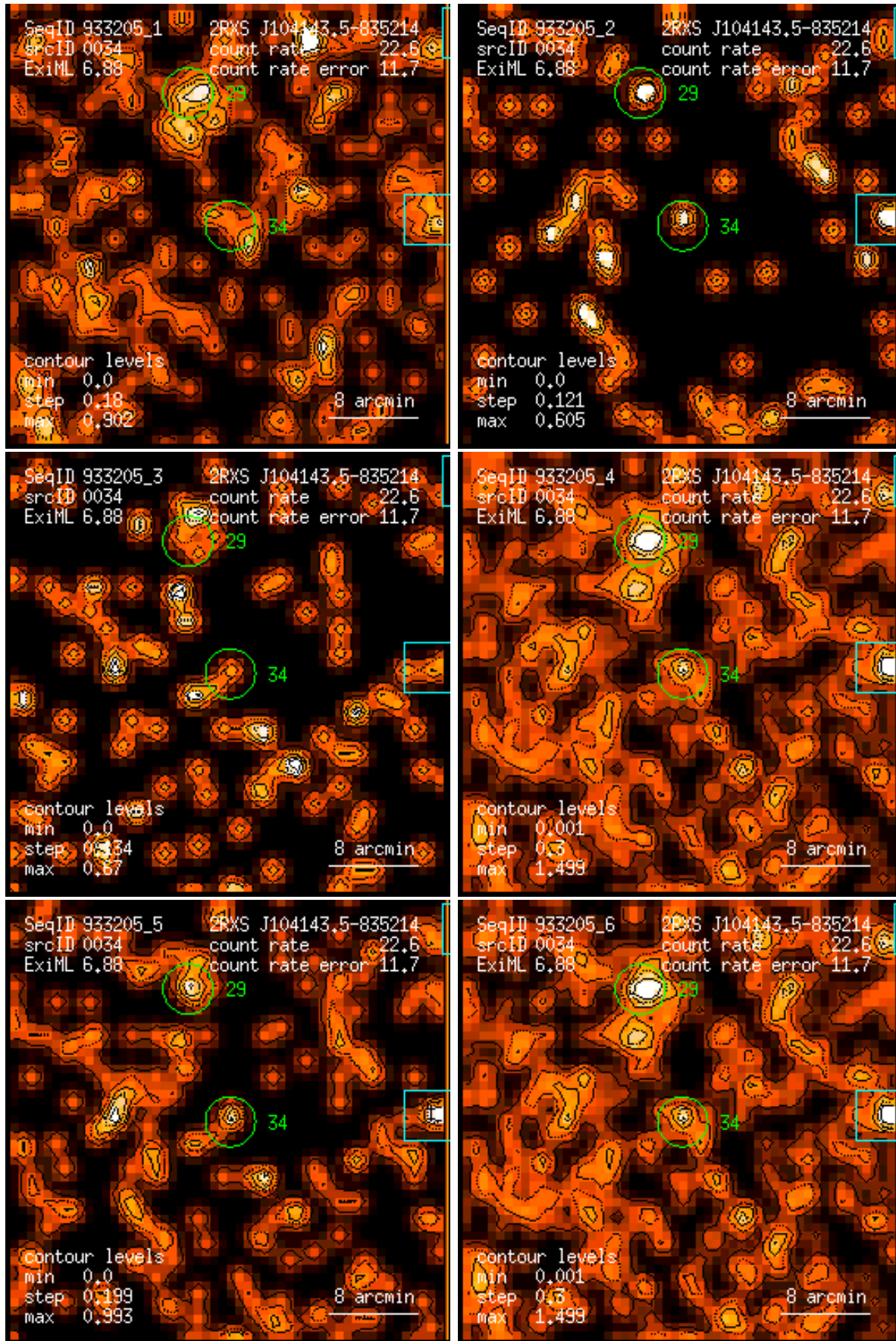
Figure 34: RASS 933205: detection 0034: band rate images, Gaussian filter: (1) PSPC channels 11 – 41, (2) 52 – 90, (3) 91 – 201, (4) 11 – 235, (5) 52 – 201, (6) 11 – 201. Broad band rates in counts/ks. Band rate contour levels in counts/ks/arcmin 2 .
