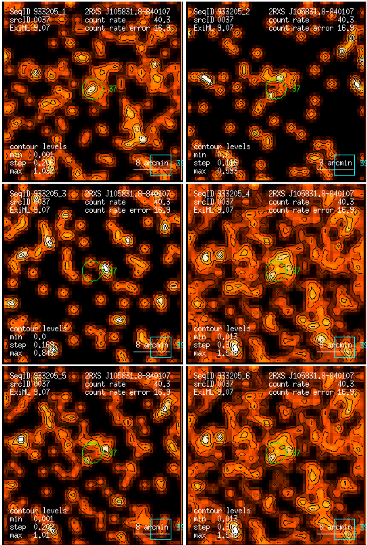
Figure 37: RASS 933205: detection 0037: band rate images, Gaussian filter: (1) PSPC channels 11 – 41, (2) 52 – 90, (3) 91 – 201, (4) 11 – 235, (5) 52 – 201, (6) 11 – 201. Broad band rates in counts/ks. Band rate contour levels in counts/ks/arcmin 2 .
