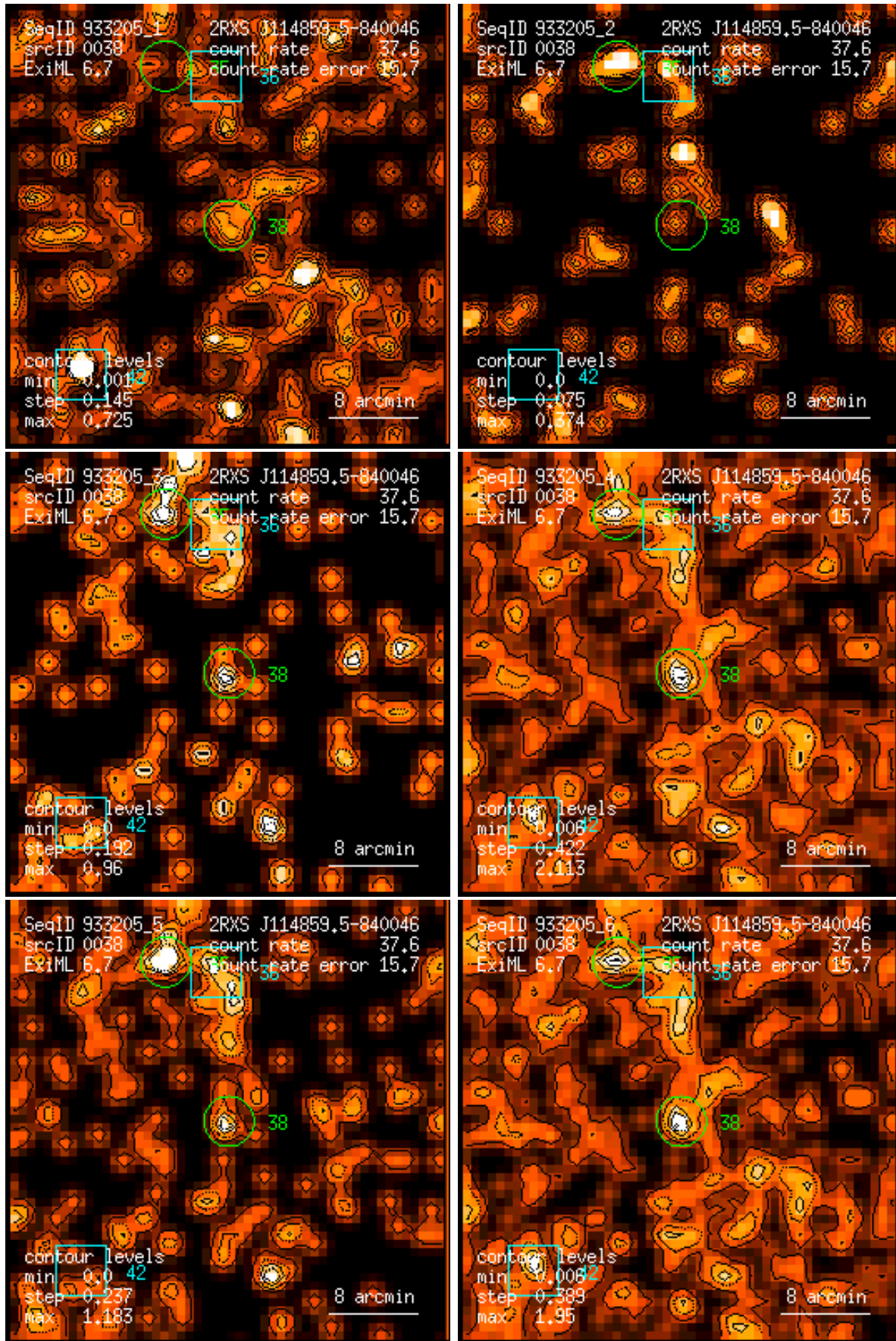
Figure 38: RASS 933205: detection 0038: band rate images, Gaussian filter: (1) PSPC channels 11 – 41, (2) 52 – 90, (3) 91 – 201, (4) 11 – 235, (5) 52 – 201, (6) 11 – 201. Broad band rates in counts/ks. Band rate contour levels in counts/ks/arcmin 2 .
