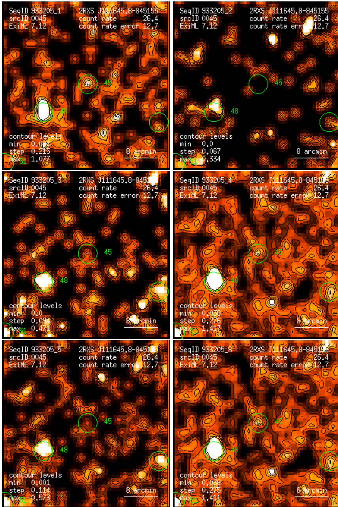
Figure 45: RASS 933205: detection 0045: band rate images, Gaussian filter: (1) PSPC channels 11 – 41, (2) 52 – 90, (3) 91 – 201, (4) 11 – 235, (5) 52 – 201, (6) 11 – 201. Broad band rates in counts/ks. Band rate contour levels in counts/ks/arcmin 2 .
