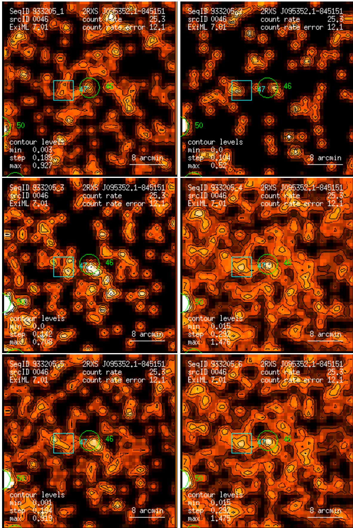
Figure 46: RASS 933205: detection 0046: band rate images, Gaussian filter: (1) PSPC channels 11 – 41, (2) 52 – 90, (3) 91 – 201, (4) 11 – 235, (5) 52 – 201, (6) 11 – 201. Broad band rates in counts/ks. Band rate contour levels in counts/ks/arcmin 2 .
