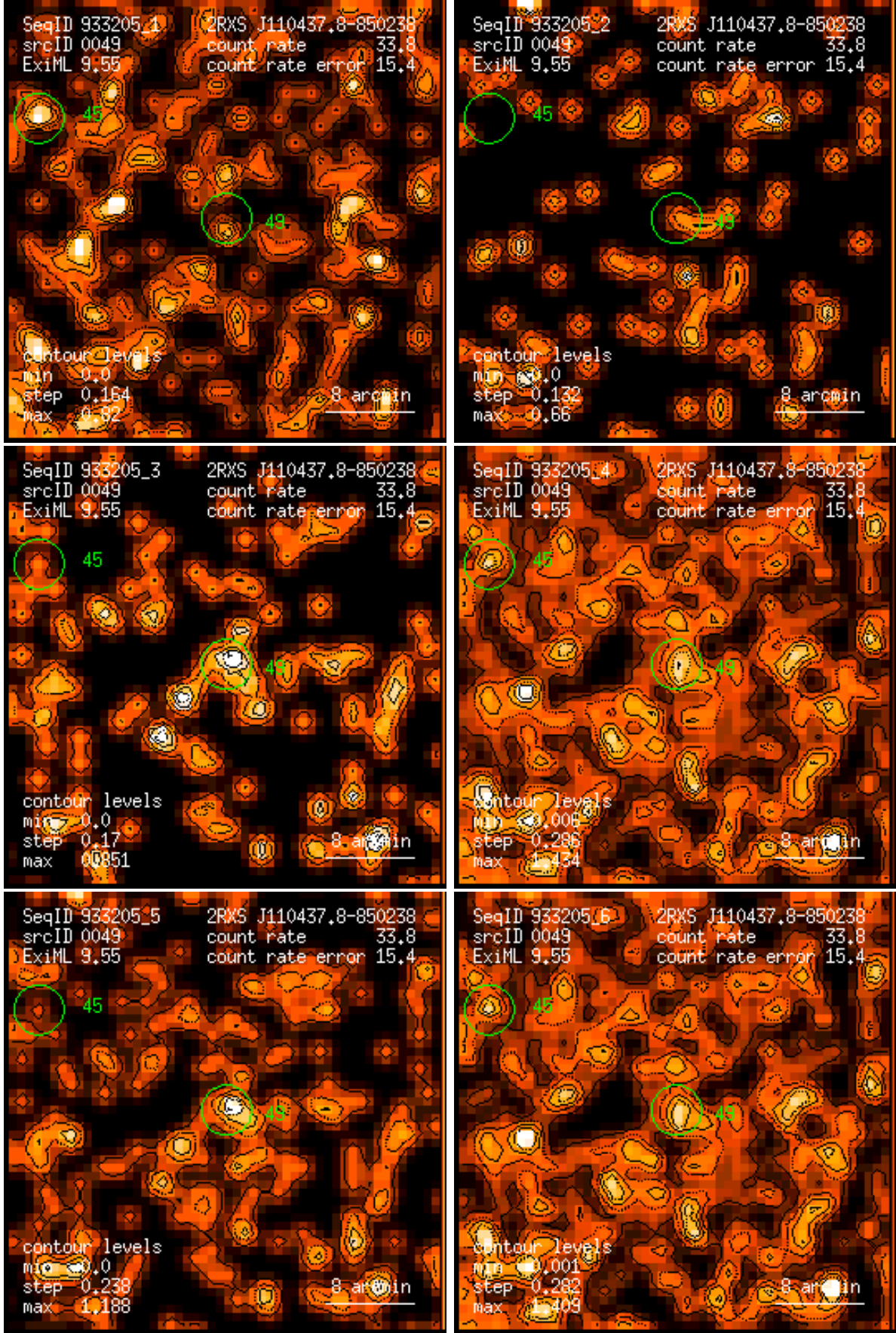
Figure 49: RASS 933205: detection 0049: band rate images, Gaussian filter: (1) PSPC channels 11 – 41, (2) 52 – 90, (3) 91 – 201, (4) 11 – 235, (5) 52 – 201, (6) 11 – 201. Broad band rates in counts/ks. Band rate contour levels in counts/ks/arcmin 2 .
