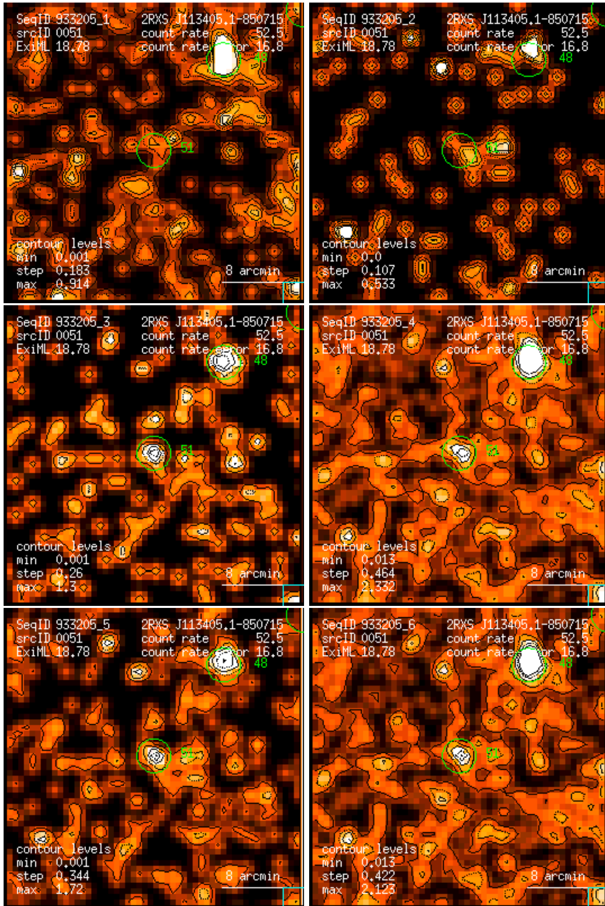
Figure 51: RASS 933205: detection 0051: band rate images, Gaussian filter: (1) PSPC channels 11 – 41, (2) 52 – 90, (3) 91 – 201, (4) 11 – 235, (5) 52 – 201, (6) 11 – 201. Broad band rates in counts/ks. Band rate contour levels in counts/ks/arcmin 2 .
