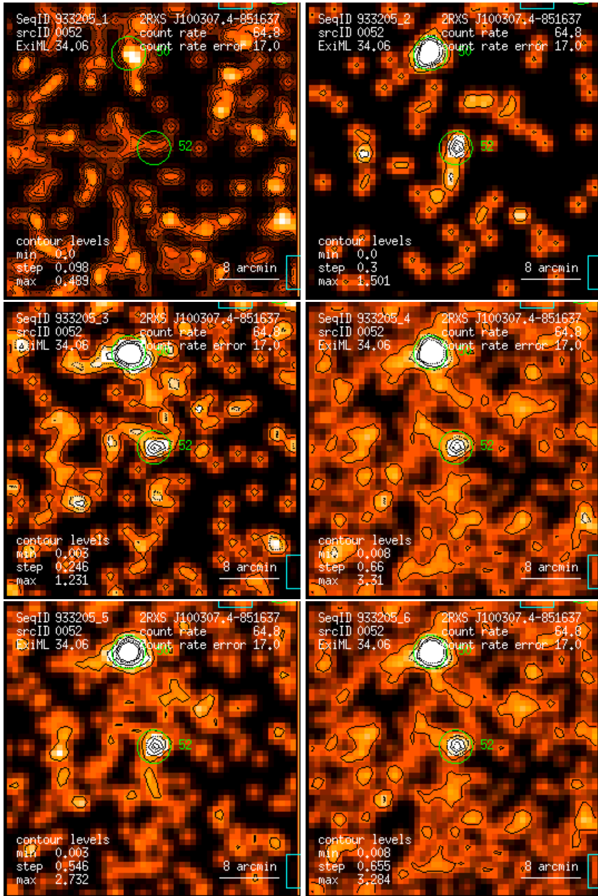
Figure 52: RASS 933205: detection 0052: band rate images, Gaussian filter: (1) PSPC channels 11 – 41, (2) 52 – 90, (3) 91 – 201, (4) 11 – 235, (5) 52 – 201, (6) 11 – 201. Broad band rates in counts/ks. Band rate contour levels in counts/ks/arcmin 2 .
